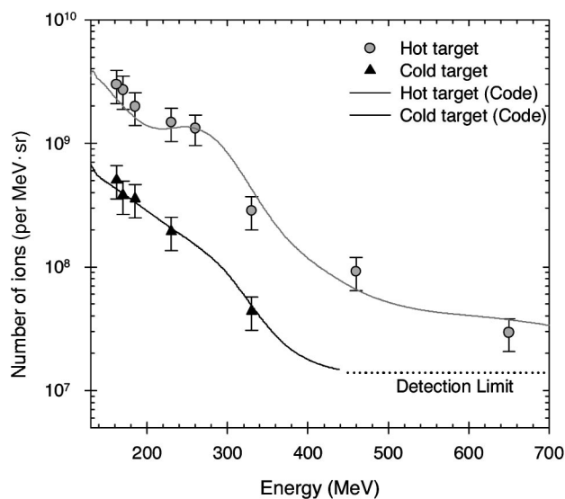
FIG. 4. Fe ion energy distribution, deduced by determining the numbers of ions (with energy above the reaction threshold energy) required to induce the measured activities of the ^{66}\text{Ge} , ^{65}\text{Ga} , ^{62}\text{Zn} , ^{66}\text{Ga} , ^{63}\text{Zn} , ^{61}\text{Cu} , and ^{57}\text{Co} nuclides. ^{60}\text{Cu} was not used in the calculations due to possible cascade contributions from the production of ^{60m}\text{Co} , for which cross sections were not available. The black and gray points result from calculations performed for each observed reaction with the Fe foil target unheated and heated to 860^\circ\text{C} respectively. The black and gray lines are the corresponding results of the full convolution involving all the above reactions. The detection limit for the technique was determined to be \sim 10^7 ions/MeV in the high energy range.
