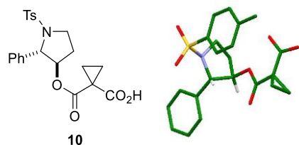
Figure 1. Single-crystal X-ray structure of pyrrolidine 10 .
