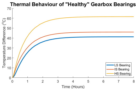
Figure 4: "Healthy" Thermal Model - Bearings
