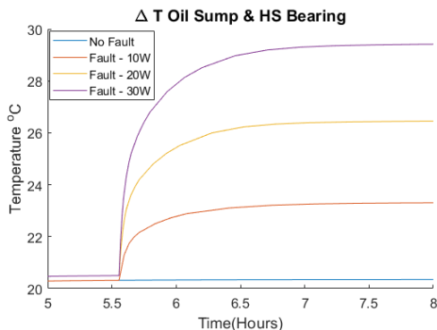
Figure 11: Temperature difference between HS bearing and Oil sump due to fault at HS bearing
