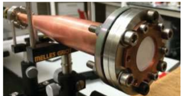
Fig. 2. A photograph of the upgraded W-band corrugated horn and output window.
