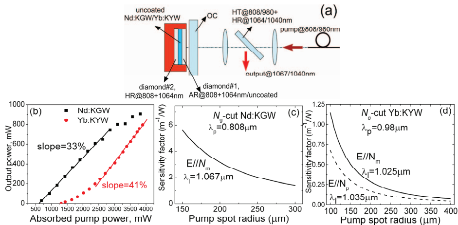
Fig. 1 (a) Quasi-microchip laser setup : OC – output coupler ; (b) output powers of Nd :KGW and Yb :KYW quasi-microchip lasers as function of absorbed pump power ; (c) calculated sensitivity factor of thermal lens in N_g -cut Nd:KGW crystals for light polarisation along N_m axis; (d) calculated sensitivity factor of thermal lens in N_g -cut Yb:KYW crystals for light polarisation along N_m and N_p axes.
