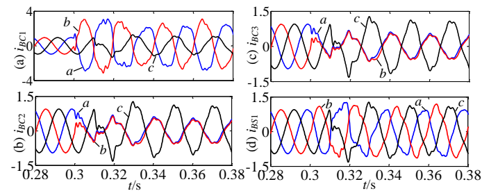
Fig. 9. Three phase currents flowing through circuit breakers during asymmetrical solid fault F2: (a) cluster breaker B_{C1} , (b) cluster breaker B_{C2} , (c) cluster breaker B_{C3} , and (d) string breaker B_{S1} .
