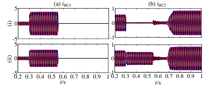
Fig. 12. Overcurrent protection during symmetrical cluster cable fault F2 with short-circuit resistance of: (i) 1 p.u. and (ii) 10 p.u.: (a) currents of breaker B_{C1} on the faulty cable and (b) currents of breaker B_{C2} on the healthy cable.
