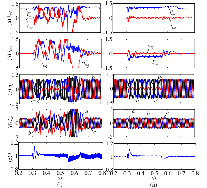
Fig. 6. Simulation results during asymmetrical solid fault F1 (i) without and (ii) with negative-sequence current controller: (a) positive- and negative-sequence d -axis currents, (b) positive- and negative-sequence q -axis currents, (c) three-phase voltages, (d) three-phase currents, and (e) offshore frequency.
