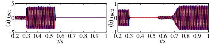
Fig. 8. Three phase currents flowing through circuit breakers during symmetrical cluster cable solid fault F2: (a) breaker B_{C1} on the faulty cable and (b) breaker B_{C2} on the healthy cable.
