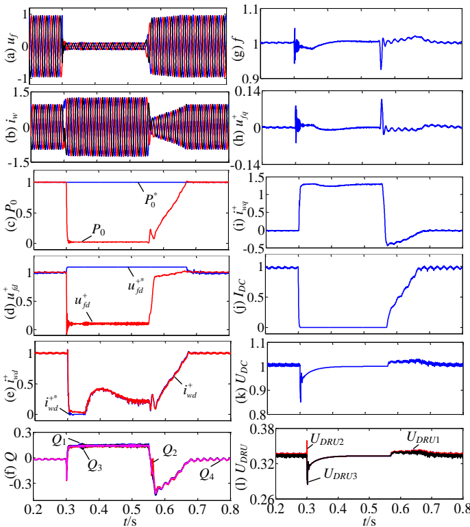
Fig. 5. Simulation results during symmetrical solid fault F1: (a) three-phase voltages, (b) three-phase currents, (c) active power, (d) d -axis voltage, (e) d -axis current, (f) reactive power, (g) frequency, (h) q -axis voltage, (i) q -axis current, (j) DRU-HVDC link current, (k) DRU-HVDC link voltage, and (l) DRU voltages.
