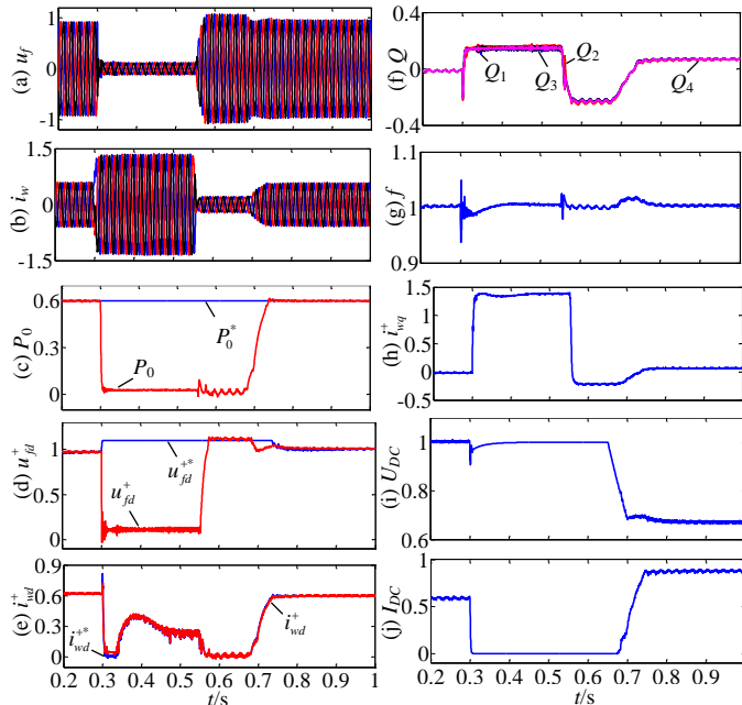
Fig. 7. Waveforms of reduced DC voltage operation during symmetrical solid fault F2: (a) three-phase voltages, (b) three-phase currents, (c) active power, (d) d -axis voltage, (e) d -axis current, (f) reactive power, (g) frequency, (h) q -axis current, (i) DRU-HVDC link voltage, and (j) DRU-HVDC link current.
