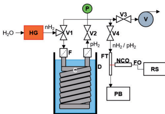
Figure 1. Schematic of the in-house built \text{pH}_2 generator. \text{H}_2 gas at 4 bar for at-line experiments, or 5 bar for on-line experiments (as shown in figure), was produced from water using a hydrogen generator (HG) electrolysis cell. The gas flowed into a two-way valve (V1), which directed the gas into either a chamber for enrichment of the \text{pH}_2 content or directly into the rest of the system. The chamber for the enrichment of \text{pH}_2 content is a copper coil (C) (OD = 9.5 mm, ID = 7.7 mm, L = 3 m) packed with charcoal, which was submerged in a Dewar (D) filled with liquid nitrogen. The charcoal was held in place with two 40\ \mu\text{m} in-line filters (F) at either end of the coil. On-off valves (V2, V3, V4) were used to control whether \text{nH}_2 - or \text{pH}_2 -enriched gas was provided to the outlet of V4. The system pressure was measured using a pressure transducer (P). A vacuum pump (V) was used to allow the system (and any connected flow tube (FT) or NMR tube) to be evacuated of gas.
