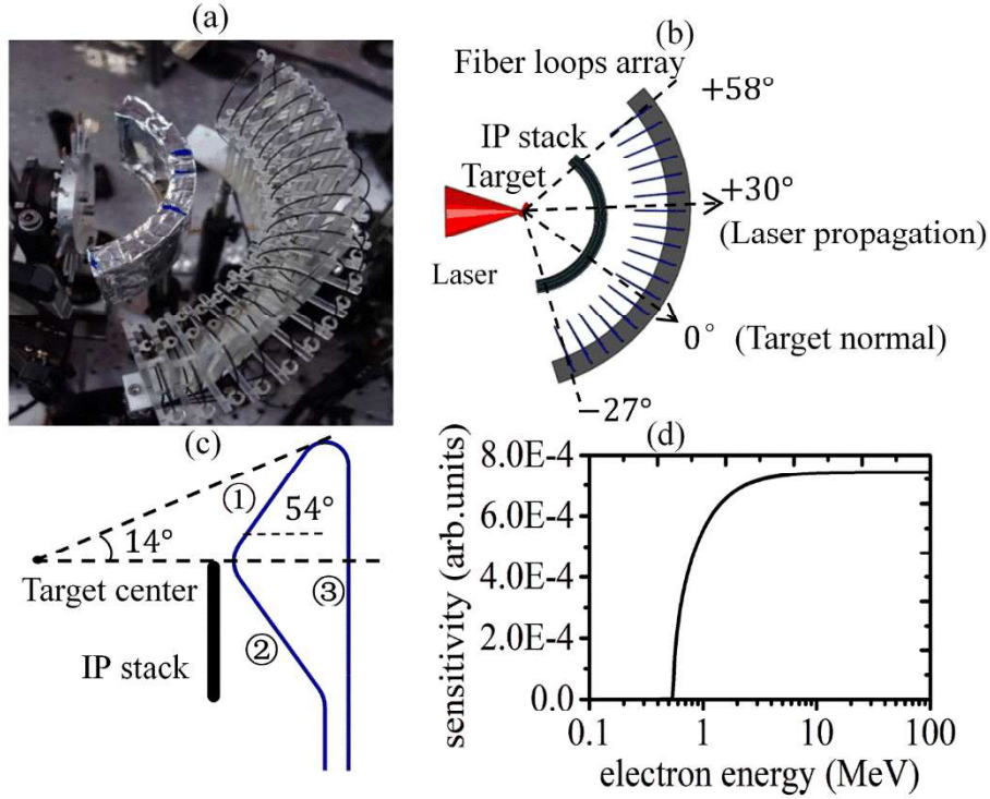
FIG. 6. (a) Photograph of the experimental layout of angular distribution measurement using IP stacks and a fibre loop array. (b) Schematic top view of the layout in (a). (c) Schematic diagram of the setup of the curved fibre loop. (d) Energy dependent sensitivity of the curved fibre loop in (c).
