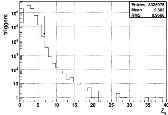
Figure 3. Distribution of Z_g values for all WaveBurst triggers. The arrow shows the location of the initial significance cut, Z_g > 6.7 .
