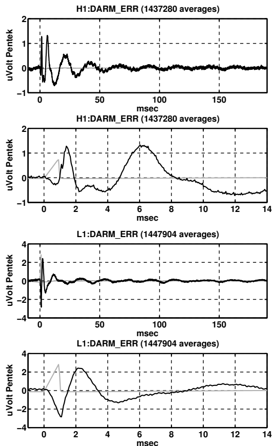
FIG. 1: Periodic timing transient in the gravitational wave channel (DARM_ERR), calibrated in \mu Volt at the ADC (Pentek card) for H1 (top two) and L1 (bottom two) shown with a span of 200 msec and 14 msec in black. The x-axis is the offset from a full GPS second. About 1.4 million seconds of DARM_ERR data was averaged to get this trace. Also shown in gray is the GPS_RAMP signal that was used as a timing monitor. It was identified as a cause of the periodic timing transient in DARM_ERR. The H1 trace shows an additional feature at 6 msec.
