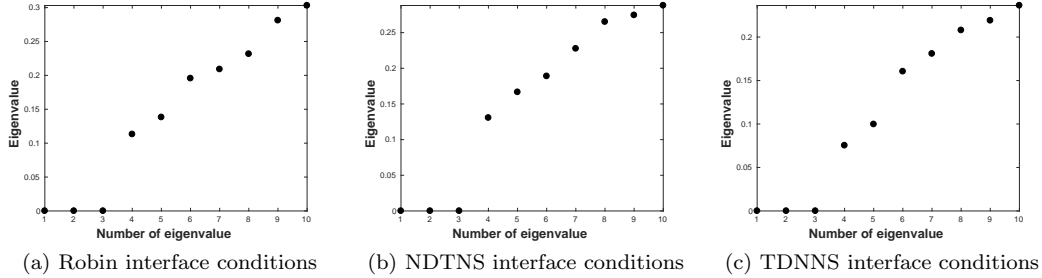
Figure 4: Eigenvalues on one of the floating subdomains in case of uniform decomposition and Taylor-Hood discretisation (\mathbf{TH}_h^3, R_h^2) - the L-shaped domain problem.
