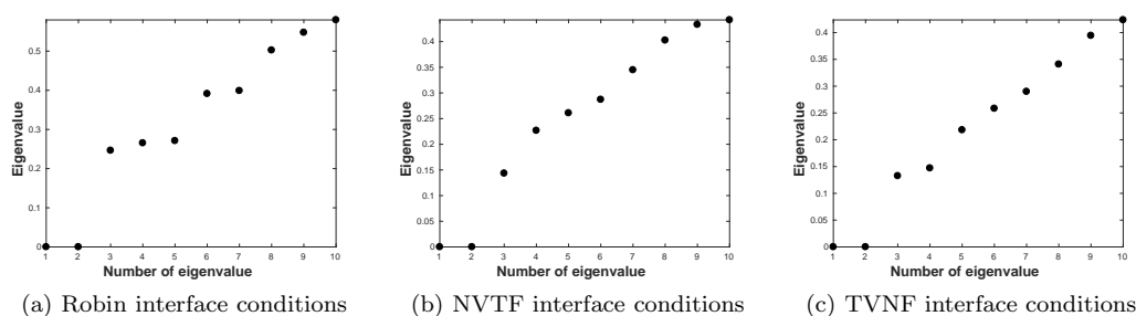
Figure 8: Eigenvalues on one of the floating subdomains in case of uniform decomposition and Taylor-Hood discretisation (\mathbf{TH}_h^2, R_h^1) - the driven cavity problem.
