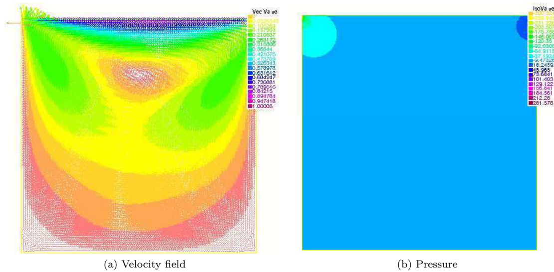
Figure 7: Numerical solution of the driven cavity problem - the driven cavity problem.
