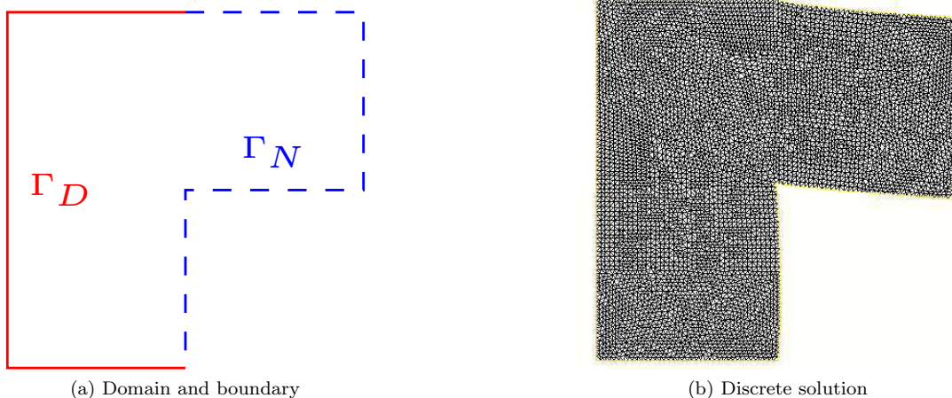
Figure 3: L-shaped domain problem.
