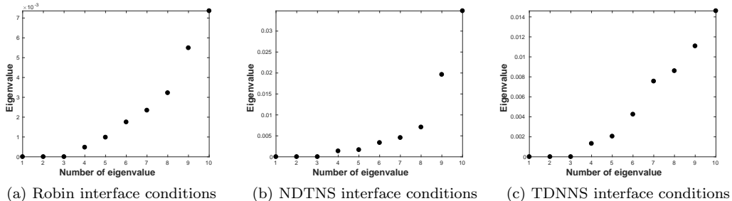
Figure 6: Eigenvalues on one of the floating subdomains in case of METIS decomposition and Taylor-Hood discretisation (\mathbf{TH}_h^3, R_h^2) - the heterogeneous beam.
