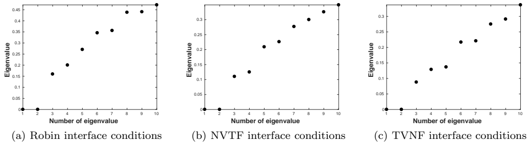
Figure 10: Eigenvalues on one of the floating subdomains in case of METIS decomposition and Taylor-Hood discretisation (\mathbf{TH}_h^3, R_h^2) - the T-shaped problem.
