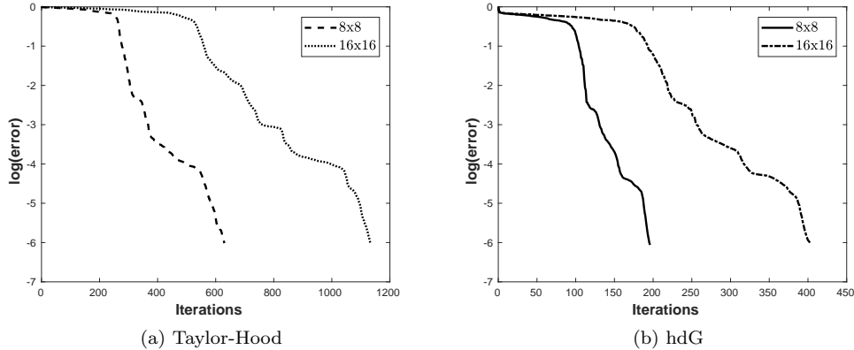
Figure 1: Increase of the size of the plateau region for increasing number of subdomains.
