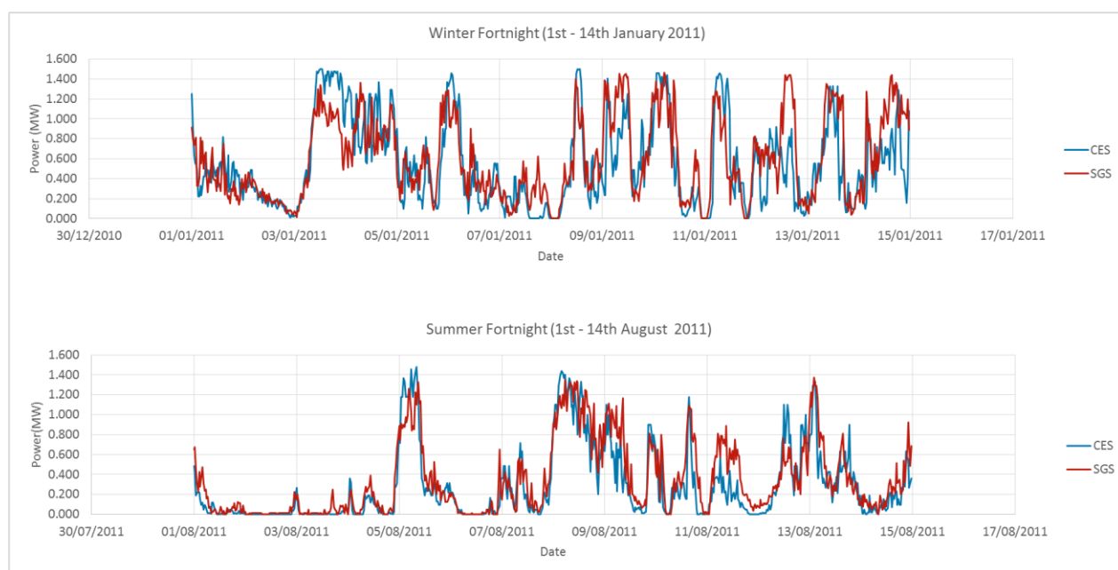
Figure 4: Comparison of Data set-SGS vs. Data set-CES time-series of Ferneylea uncurtailed output
