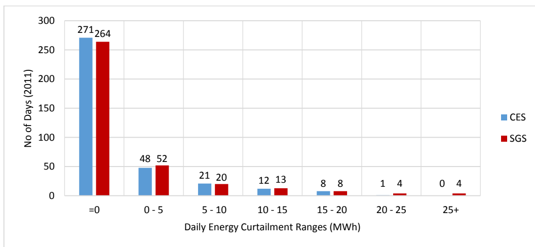
Figure 6: Daily energy curtailment rate of Ferneylea wind farm
