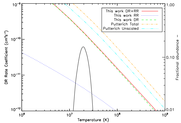
Figure 10. Same as Figure 9, but for 42-like.
