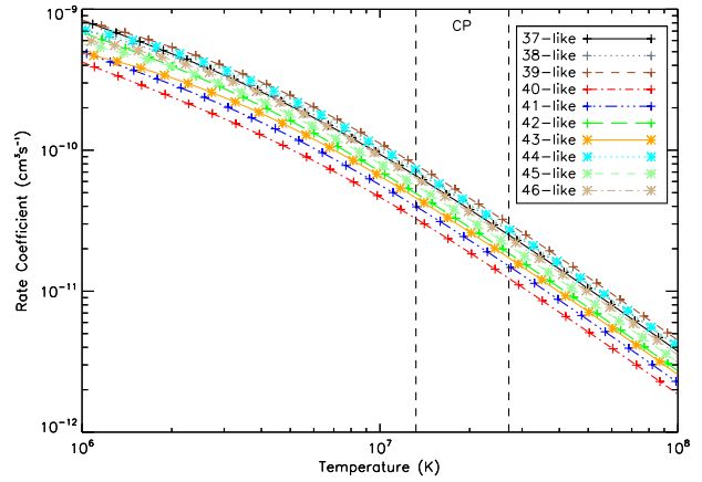
Figure 4. Total DR rate coefficients for the 4-5 core excitation for 37- to 46-like, calculated in IC.
