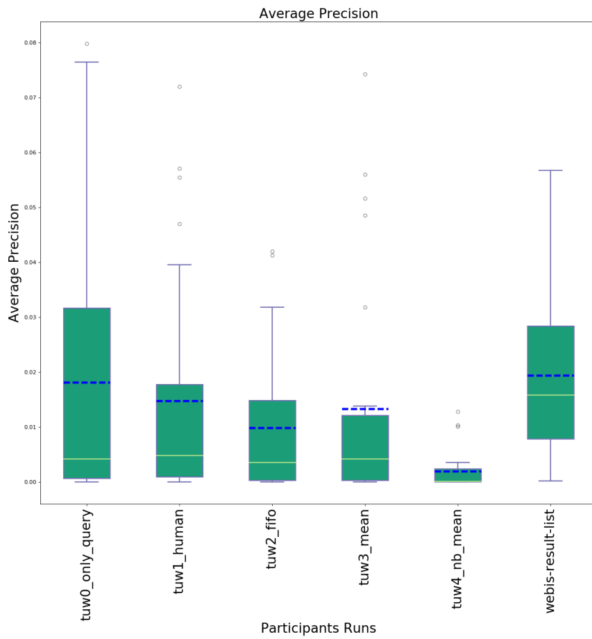
Fig. 1. Box-plots of average precision values across the topics; the blue dashed line represents the mean average precision.
