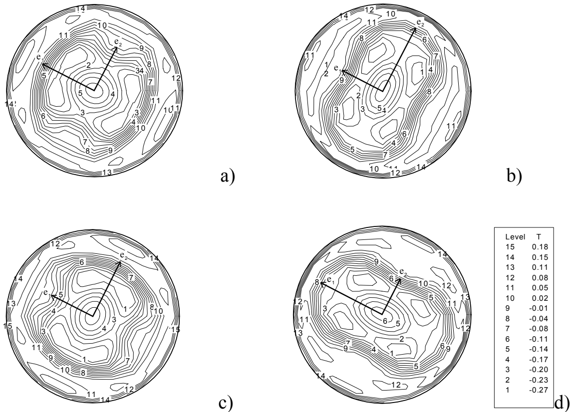
Fig. 14: Temperature distribution in the section z=0.75 for A=0.4 ( Ma=3.6 \cdot 10^4 ) and standing wave regime (the field is shown in figs a,b,c,d corresponding to t=0, \tau/4, \tau/2, 3\tau/4 )
