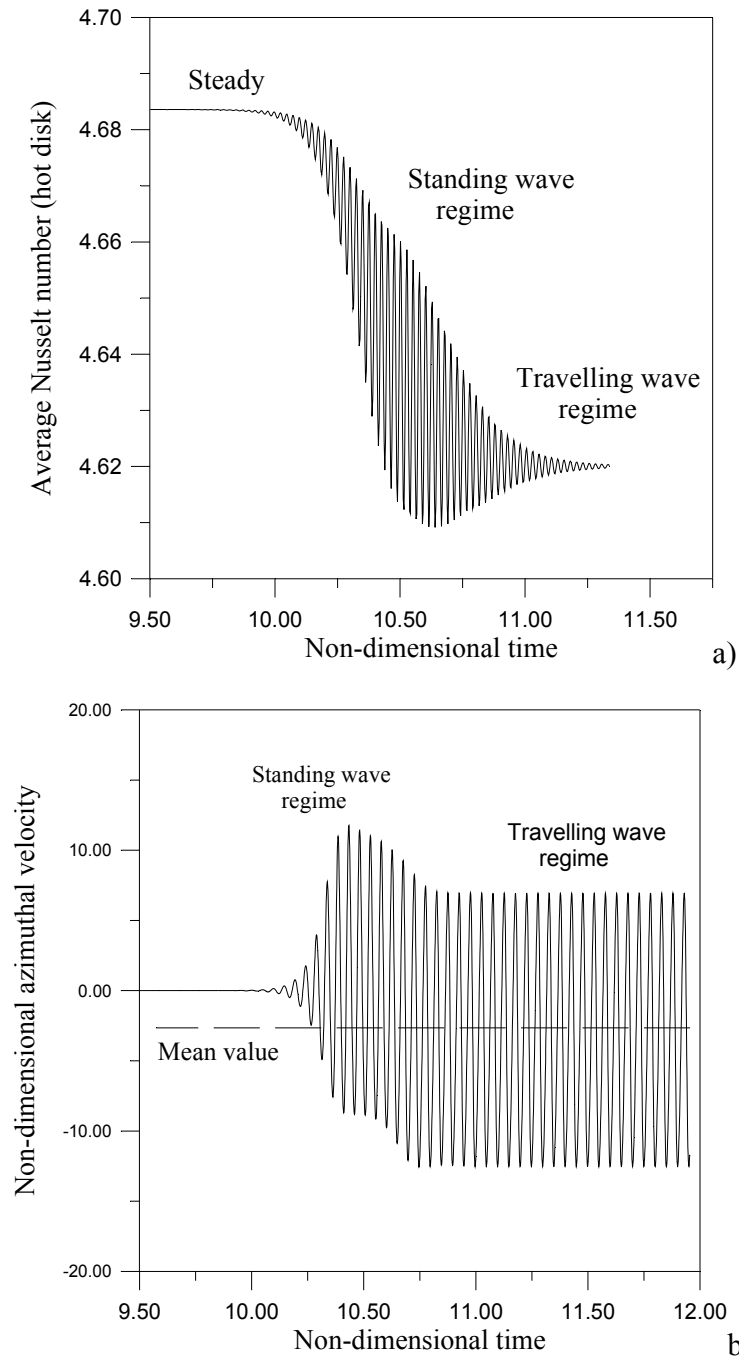
Fig. 24: (a) Average Nusselt number on the hot disk in the case A=0.5 , Pr=4 , Ma=4800 , (b) azimuthal velocity in the point z=0.75 , r=0.5 , \phi=0 for A=0.5 , Pr=4 , Ma=4800 .
