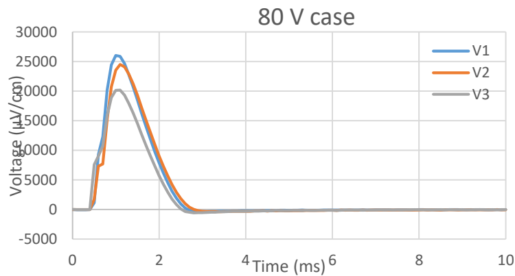
Figure 9. Voltage Drop Across the tapes for 80 V Discharge Test.
