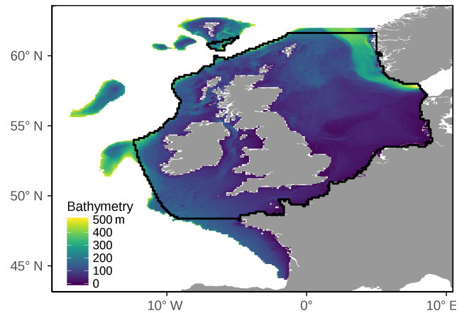
Figure 1. Region where the sedimentary environment was mapped. We defined the north-west European Shelf as the region between 17° W and 9° E and 44 and 63° N, where bathymetry was less than 500 m. The solid black line demarcates the region where tidal velocities were taken from the Scottish Shelf Model, as described in Sect. 2.2.4.
