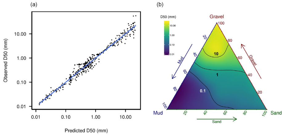
Figure 6. (a) Predictions of a GAM that relates whole-sediment D 50 to the mud, sand and gravel percentages. (b) Relationship between total sediment median grain size and percentage of mud, sand and gravel. The relationship was derived using a general additive model which relates the D 50 to the mud, sand and gravel percentage.
