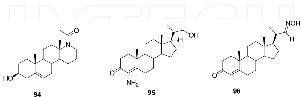
Figure 8. Other steroidal inhibitors of CYP17.
