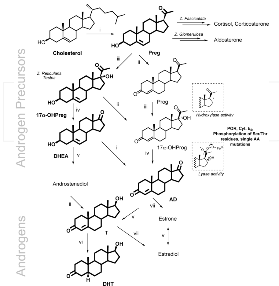
Figure 2. CYP17 and androgen physiology. i. P450 cholesterol side-chain cleavage (P450 scc ); ii. 3 \beta -Hydroxysteroid dehydrogenase, \Delta^4 -isomerase; iii. CYP17 (OHase); iv. CYP17 (lyase); v. 17 \beta -Hydroxysteroid dehydrogenase; vi. 5 \alpha -Reductase; vii. Aromatase (CYP19).
