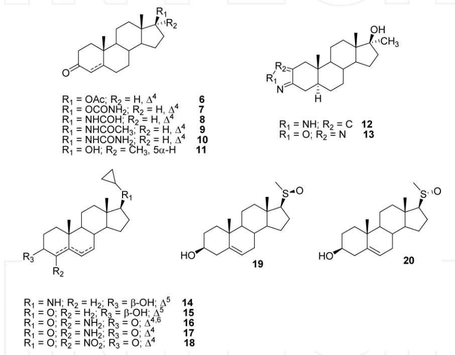
Figure 3. Androstane based CYP17 inhibitors.
