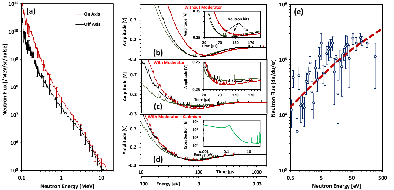
FIG. 3. (a) Typical spectrum of fast neutrons produced in the experiment, as measured by the ND-1 (on-axis) and ND-2 (35° off axis) detectors. (b), (c) Raw data (from three shots for each case) obtained in the ^3\text{He} detectors without and with the moderator, respectively. (d) Raw data in presence of the moderator obtained in the ^3\text{He} detectors wrapped with Cd foil, which is a good absorber of neutrons of energies below \sim 0.5 eV, as can be seen from the cross-section of ^{113}\text{Cd}(n,\text{total}) [20] plotted in the insert. The zoomed plots of the raw data in linear X-scale are shown in the inserts. Epithermal neutron hits are identified by the voltage spikes in the output signal (as shown in the insert in (b)) and the neutron energy is calculated by ToF (as shown in a separate axis under (d)). (e) Epithermal neutron spectra produced by the moderator, averaged over 16 measurements, where the red line is a eye-guide to the data points.
