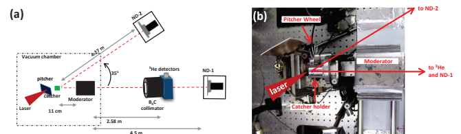
FIG. 1. (a) Schematic of the experimental setup (figure not to scale). (b) Image of the setup inside the interaction chamber. The fast neutrons were generated by nuclear reactions in the catcher target induced by the MeV ions accelerated from the laser irradiated pitcher target. ND-1 and ND-2 are EJ232Q scintillator detectors, placed inside lead and plastic housings, employed in ToF mode to diagnose the fast neutron spectra[18]. Epithermal neutrons produced by the moderator were diagnosed by the ^3\text{He} proportional counters employed in ToF mode, placed behind a \text{B}_4\text{C} collimator.
