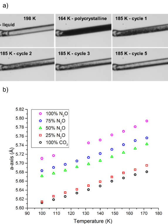
Figure 4: a) Condensing and annealing crystallisation of 50:50 mixture of CO 2 /N 2 O; cycle 4 was omitted as it did not show a substantial visual change from cycle 3. b) Unit cell parameters for various ratios of solid solutions as a function of temperature.
