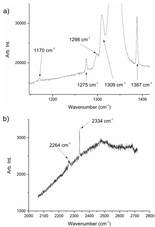
Figure 1: Raman spectra of the decomposition products showing peaks associated with both \text{CO}_2 and \text{N}_2\text{O} . The peaks at 1275, 1309, 1387, 2334 \text{cm}^{-1} are representative of \text{CO}_2 22 whilst those at 1170, 1298, 2264 \text{cm}^{-1} are representative of \text{N}_2\text{O} . 23 The large peak at \sim 1350 \text{ cm}^{-1} is from the diamond anvils. The high fluorescence can be attributed to the diamond anvils however there may have been contributions from residual yellow reaction deposits present in the cell.
