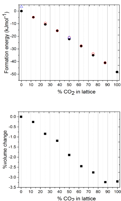
Figure 5 (a) Graph of relative lattice energy versus %CO 2 doping in N 2 O crystal lattice, as obtained by DFT-D. Open red circles: most heterogeneously packed lattice, filled black circles: most homogeneously packed lattice. Open blue triangles: half of the N 2 O molecules from the lowest energy lattice randomly switched with respect to terminal N/O identity. Bottom: Graph of percentage unit cell volume change with increasing CO 2 doping in N 2 O crystal lattice.
