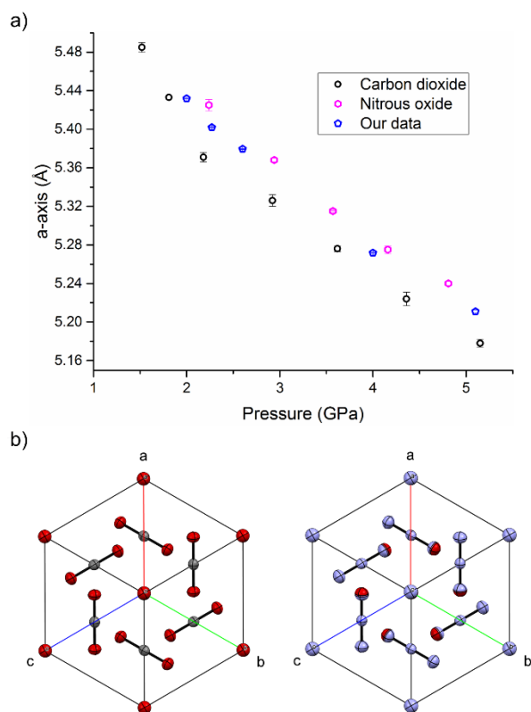
Figure 2. a) The compression of the solid solution of carbon oxide and nitrous oxide at ambient temperature, together with values of previous studies of the pure components. 25, 33 b) the isostructurality of carbon dioxide (left) and nitrous oxide (right) looking down the [111] direction.
