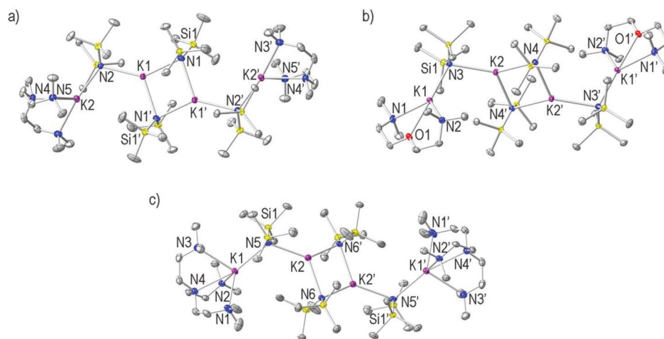
Fig. 5 (a) Molecular structures of [(KHMSD) 2 {(PMDTA·KHMSD) 2 }] 7 , (b) [(KHMSD) 2 {(TMDAE·KHMSD) 2 }] 8 and (c) [(KHMSD) 2 {(Me 6 TREN·KHMSD) 2 }] 9 . Hydrogen atoms and one toluene molecule of crystallisation for 9 are omitted for simplicity. Displacement ellipsoids are displayed at 35% probability. Selected bond distances (Å) and angles (°): for 7 , K1–N1 2.8236(13), K1–N1' 2.8452(13), K1–N2 2.8808(11), N1–K1' 2.8451(13), K2–N2 2.7536(12), K2–N4 2.8525(13), K2–N3 2.9035(15), K2–N5 2.9528(13), K2...C9 3.3223(17), K2...C15 3.366(3), K1–N1–K1' 84.08(3), K1–N2–K2 106.43(4), N1–K1–N1' 95.93(3), N1–K1–N2 141.54(4), N1'–K1–N2 122.13(4), N2–K2–N4 120.54(4), N2–K2–N3 131.85(4), N4–K2–N3 63.47(4), N2–K2–N5 123.17(4), N4–K2–N5 64.90(4), N3–K2–N5 102.46(4), the symmetry operation used to generate the equivalent atoms numbered with ' is -x + 1, -y + 1, -z + 1 ; for 8 , K1–O1 2.7362(10), K1–N3 2.8367(11), K1–N2 2.9579(12), K1–N1 2.9972(13), K2–N4' 2.8288(11), K2–N4 2.8660(11), K2–N3 2.9254(11), O1–K1–N3 173.68(3), O1–K1–N2 59.83(3), K1...C18' 3.3147(14), K2...C18' 3.3353(15), K2–N4–K2' 84.35(3), K2–N3–K1 108.36(3), N3–K1–N2 126.25(3), O1–K1–N1 60.04(4), N3–K1–N1 113.95(4), N2–K1–N1 119.79(4), N4'–K2–N4 95.65(3), N4'–K2–N3 121.12(3), N4–K2–N3 140.39(3), the symmetry operation used to generate the equivalent atoms numbered with ' is -x + 2, -y + 1, -z + 1 ; for 9 , K1–N5 2.913(2), K1–N2 2.919(2), K1–N1 3.003(3), K1–N4 3.018(2), K1–N3 3.048(2), N5–K2 2.906(2), K2–N6' 2.846(2), K2–N6 2.848(2), N6–K2' 2.846(2), K1...C23 3.402(3), K2...C30' 3.239(4), K2–N6–K2' 83.42(6), K2–N5–K1' 117.64(7), N5–K1–N2 119.91(6), N5–K1–N1 126.90(7), N2–K1–N1 101.57(7), N5–K1–N4 165.97(6), N2–K1–N4 62.44(6), N1–K1–N4 62.42(7), N5–K1–N3 105.29(7), N2–K1–N3 96.24(7), N1–K1–N3 101.16(8), N4–K1–N3 60.96(6), K2–N5–K1 117.64(7), N6'–K2–N6 96.58(6), N6'–K2–N5 132.40(6), N6–K2–N5 126.95(6), the symmetry operation used to generate the equivalent atoms labelled with ' is -x + 3, -y + 1, -z + 1 .
