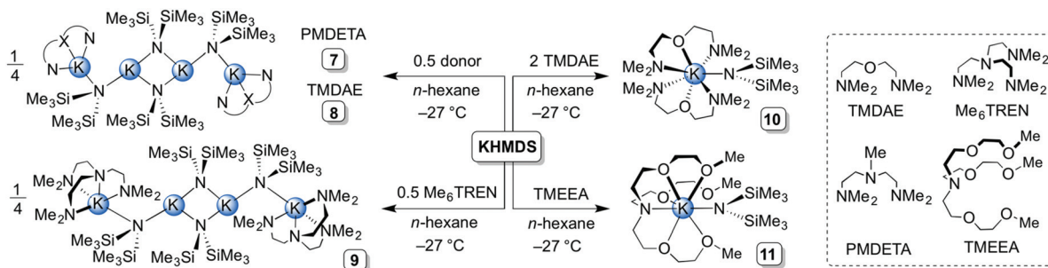
Scheme 2 Synthesis of tetranuclear [(\text{KHMDS})_2(\text{PMDETA}\text{-KHMDS})]_2 7 , [(\text{KHMDS})_2(\text{TMDAE}\text{-KHMDS})]_2 8 and [(\text{KHMDS})_2(\text{Me}_6\text{TREN}\text{-KHMDS})]_2 9 , and monomeric [\text{KHMDS}(\text{TMDAE})]_2 10 and [\text{KHMDS}(\text{TMEEA})] 11 .
