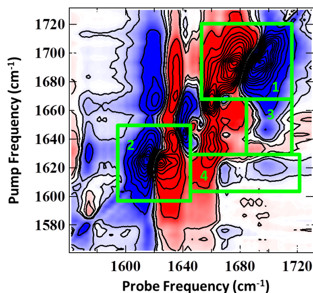
Figure 4 – Spectral distribution of 2D-IR PC2 corresponding to the temperature-induced difference spectrum associated with AT-15mer duplex melting. Arrows and highlighted regions correspond to references in the main text. Colour scale runs from red (negative) to blue (positive).
