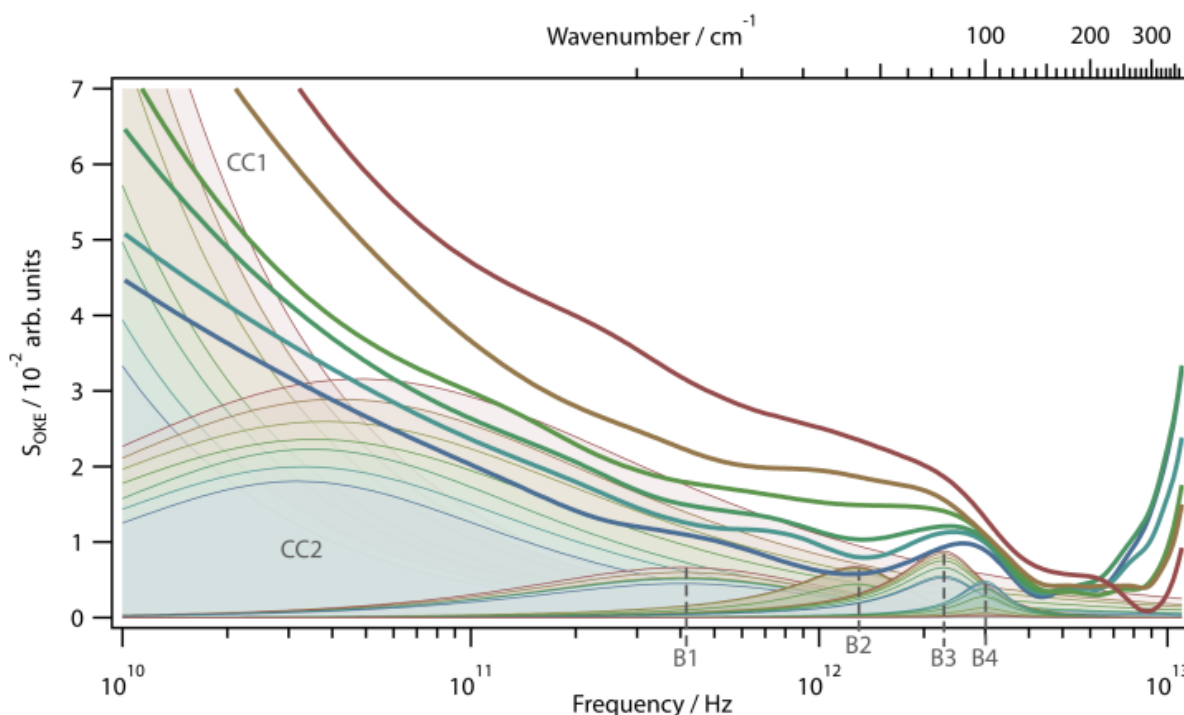
Figure 5 – Temperature-dependent OKE spectra of the AT 15-mer and the functions used to model them (filled), see text for details. The temperatures run from 298 K (blue) to 358 K (red) in intervals of 10 K.
