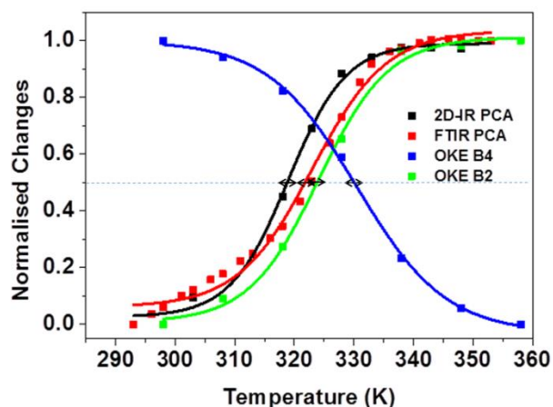
Figure 8 – Normalised melting curves for AT-15mer duplex extracted from FTIR, 2DIR and OKE experiments. Arrows show estimated inaccuracies in T_m values from experimental repeatability.
