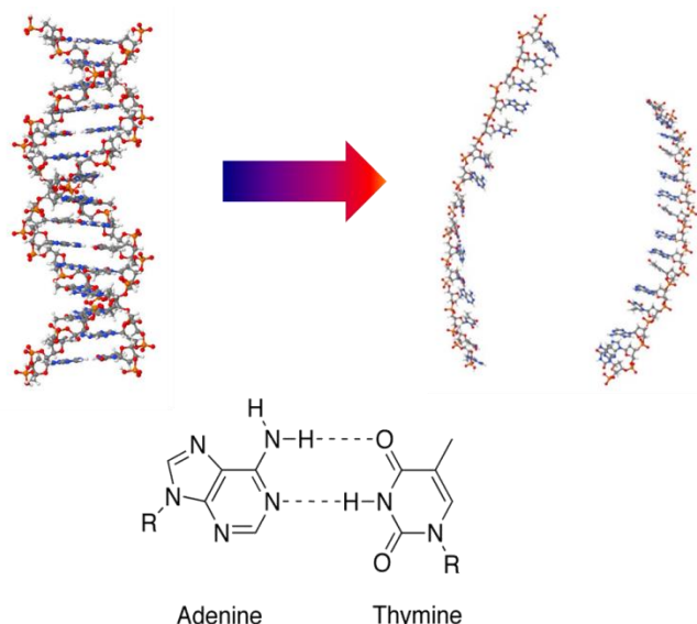
Figure 1 – Schematic diagram illustrating the thermal denaturation transition of the AT-15mer DNA (top) and structure of A-T base pair highlighting Watson-Crick hydrogen bonding (bottom). (DNA images created in Jmol: an open-source Java viewer for chemical structures in 3D. http://www.jmol.org/ )
