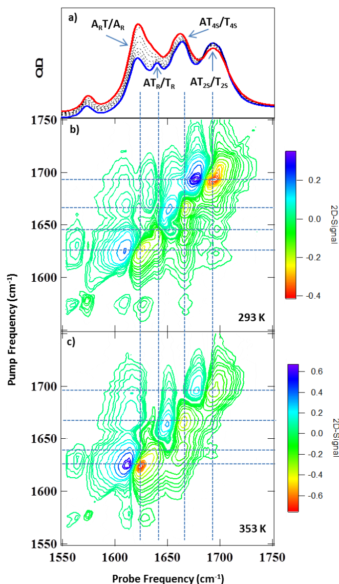
Figure 2 - a) FTIR spectra of AT 15mer duplex recorded at a range of temperatures between 293 K (blue) and 353 K (red), assignments of bands are discussed in the text. b) 2D-IR spectrum of AT 15mer at 293 K T_w = 250 fs. c) 2D-IR spectrum of AT 15mer at 353 K T_w = 250 fs. Colour scale runs from red (negative) to blue (positive) with contours at 10% intervals.
