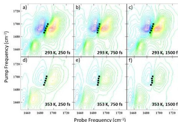
Figure 6 – 2D-IR spectra of the AT_{2S}/T_{2S} mode of the AT 15mer obtained as a function of waiting time and temperature. (a-c) show T_w = 250, 750 and 1500 fs at 293 K. (d-f) shows the same waiting times at 353 K. The black symbols show the results of a nodal line slope (NLS) analysis of the line shapes.
