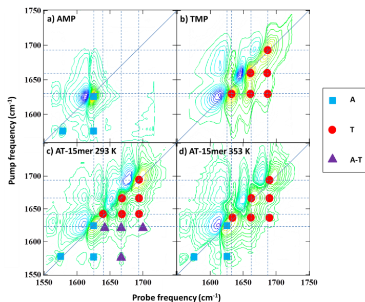
Figure 3 – 2D-IR spectra of a) AMP b) TMP and AT 15mer at c) 293 K and d) 353 K. Coloured symbols indicate the assignment of peaks visible in the AT 15mer spectra (c,d) based on the mononucleotide spectra (a,b), see text.
