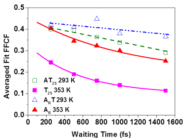
Figure 7 – Average FFCF dynamics as a function of TW for the T 2S and A R modes of the AT 15mer DNA in ds and ss conformations (see legend). Points relate to experimental data, lines show fits to exponential functions (see text).
