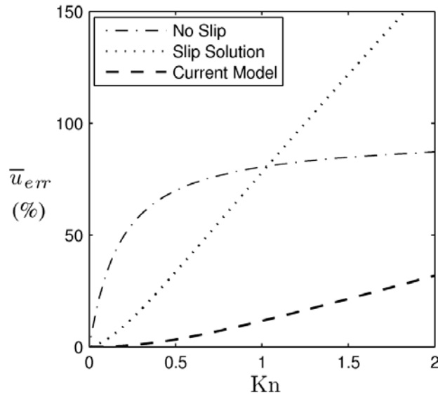
Figure 15. Average error of Poiseuille flow velocity predictions up to Kn=2.0 . Comparison of no-slip solution ( - \cdot ), slip solution ( \cdots ), and our model ( - - ). The non-dimensional applied pressure gradient is Kn .
