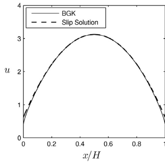
Figure 10. Non-dimensional velocity profile for Poiseuille flow, \text{Kn}=0.05 ( =\lambda/H ). Comparison of the BGK solution (—) with the slip solution (---). The non-dimensional applied pressure gradient = \text{Kn} .
