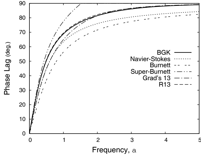
Figure 5. Velocity phase lag variation with non-dimensional body force frequency, \alpha ; \text{Kn}=0.5 . BGK solution (—); Navier-Stokes (.....); Burnett (— — —); super-Burnett (— · · —); Grad's 13 moment (— · —); Regularized 13 moment (— —).
