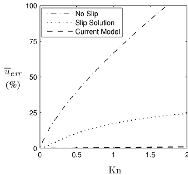
Figure 12. Average error of Couette flow velocity predictions up to Kn=2.0 . Comparison of no-slip solution ( - \cdot ), slip solution ( \cdots ), and our model ( - - ).
