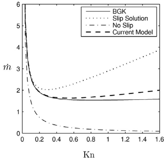
Figure 16. Normalized mass flow rate predictions for Poiseuille flow up to Kn=1.6 . Comparison of no-slip solution ( - \cdot ), slip solution ( \cdots ), BGK solutions ( - ), and our model ( - - ). The non-dimensional applied pressure gradient is Kn ; the non-dimensional mass flow rate is normalized with \sqrt{\pi}/(2Kn) .
