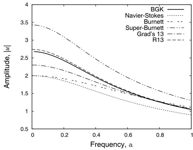
Figure 4. Wave amplitude variation with non-dimensional body force frequency, \alpha ; Kn=0.5 . BGK solution (—); Navier-Stokes (.....); Burnett (— — —); super-Burnett (— · · —); Grad's 13 moment (— · —); Regularized 13 moment (— —).
