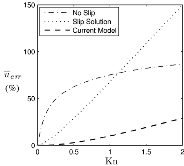
Figure 18. Average error of combined Couette/Poiseuille flow velocity predictions up to Kn=2.0 . Comparison of no-slip solution ( - \cdot - ), slip solution ( \cdots ), and our model ( - - ). The non-dimensional applied pressure gradient is Kn .
