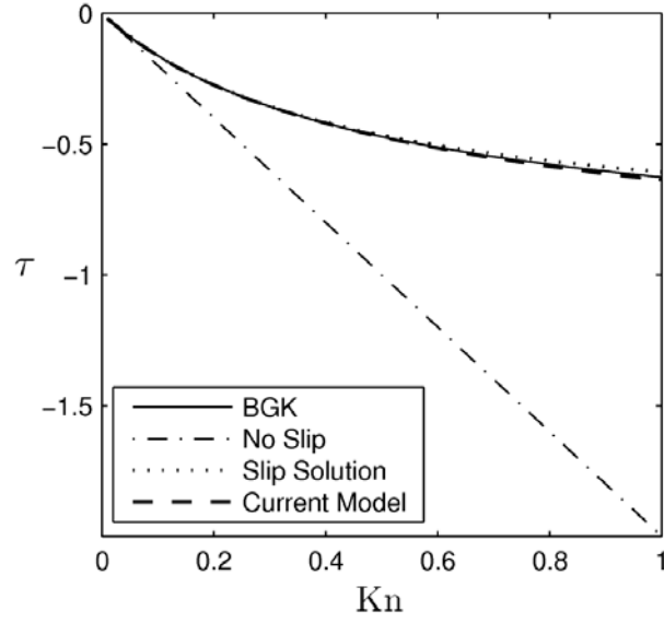
Figure 13. Non-dimensional Couette flow shear stress up to Kn=1.0 . Comparison of the no-slip solution ( - \cdot ), slip solution ( \cdots ), and our model ( - - ). The non-dimensional wall velocities at x=0 and x=H are -1 and 1 , respectively.
