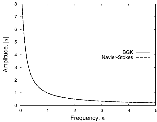
Figure 2. Wave amplitude variation with non-dimensional body force frequency, \alpha ; \text{Kn}=0.1 ; BGK solution (—); Navier-Stokes (— —).
