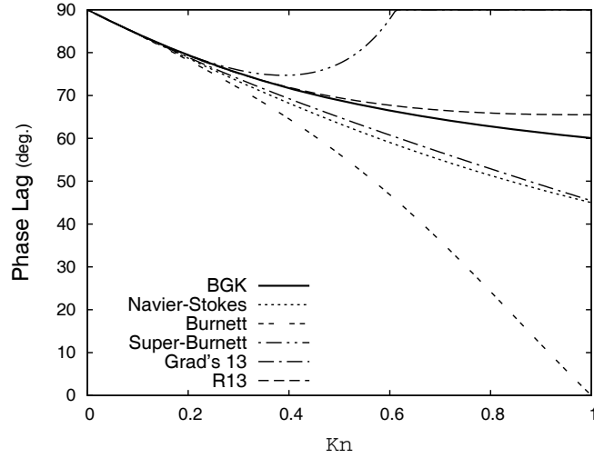
Figure 7. Velocity phase lag variation with Knudsen number; \alpha=1.0 . BGK solution (—); Navier-Stokes (.....); Burnett (— — —); super-Burnett (— · · —); Grad's 13 moment (— · —); Regularized 13 moment (— —).
