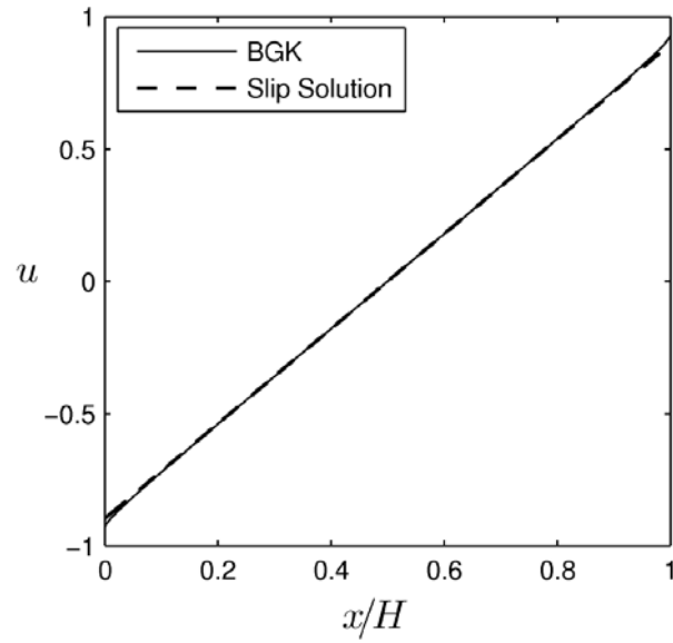
Figure 9. Non-dimensional velocity profile for Couette flow, \text{Kn}=0.05 ( =\lambda/H ). Comparison of the BGK solution (—) with the slip solution (---). Non-dimensional wall velocities at x=0 and x=H are -1 and 1 , respectively.
