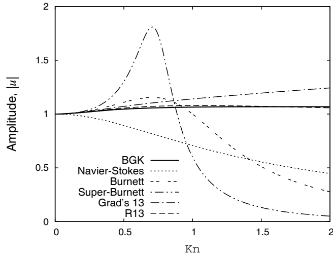
Figure 6. Wave amplitude variation with Knudsen number; \alpha=1.0 . BGK solution (—); Navier-Stokes (.....); Burnett (— — —); super-Burnett (— · · —); Grad's 13 moment (— · —); Regularized 13 moment (— —).
