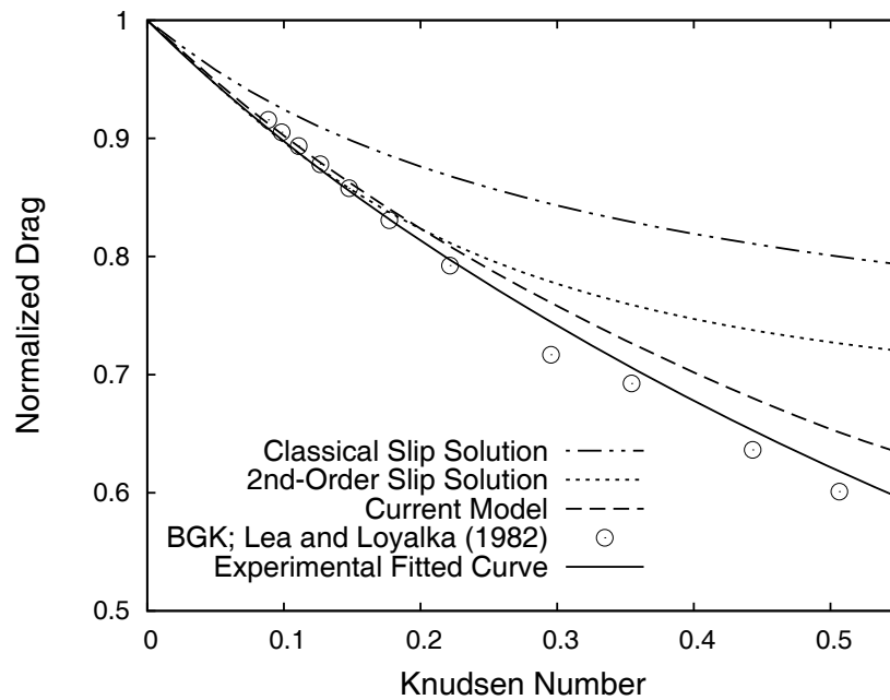
Figure 20. Normalized drag on a sphere versus Knudsen number. Comparison of classical slip solution ( -\cdot-\cdot- ) by Basset (1888); a second-order slip solution ( \cdots ) by Cercignani (1990); our model ( - - ); a BGK solution by Lea & Loyalka (1982); and a curve fit to the experimental data of Allen & Raabe (1985).
