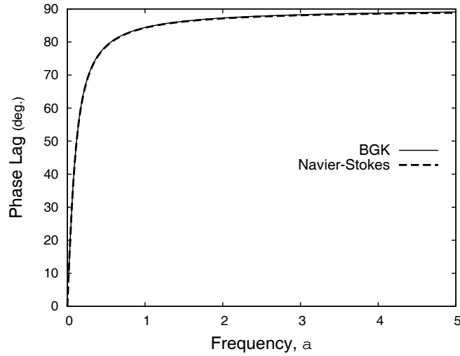
Figure 3. Velocity phase lag variation with non-dimensional body force frequency, \alpha ; Kn=0.1 ; BGK solution (—); Navier-Stokes (---).
