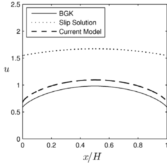
Figure 14. Non-dimensional velocity profile for high-Knudsen-number Poiseuille flow ( Kn=1.0 ). Comparison of the slip solution ( \cdots ), the BGK solution ( - ), and our model ( - - ). The non-dimensional applied pressure gradient is Kn .
