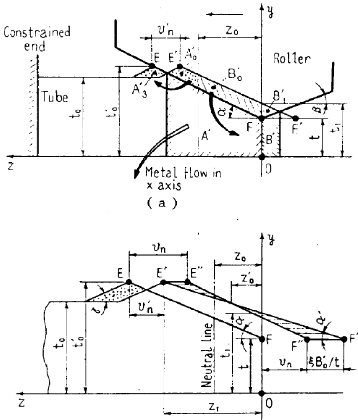
Figure 4 Mechanism of plastic flow in backward flow forming
