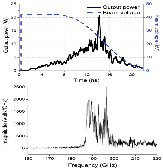
Fig. 3 BWO output power (top) and frequency spectrum (bottom) as predicted using 2D PIC code MAGIC
