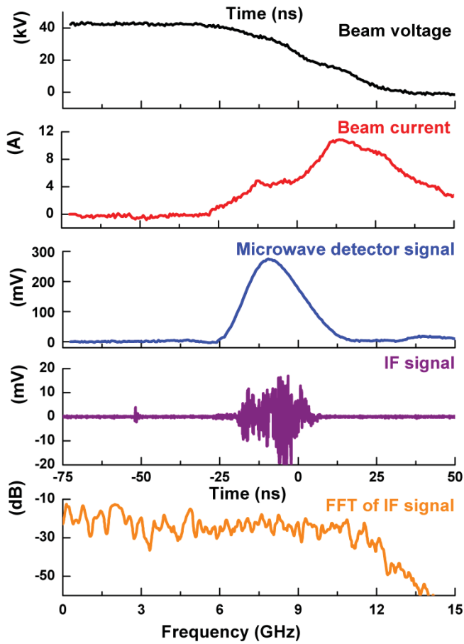
Fig. 4 Time-correlated electron beam voltage, current pulse, the millimetre wave pulse from the 200 GHz BWO, the intermediate frequency (IF) output from a harmonic mixer recorded on a deep memory (20 GHz) single shot digital storage oscilloscope and FFT result of the intermediate frequency output.
