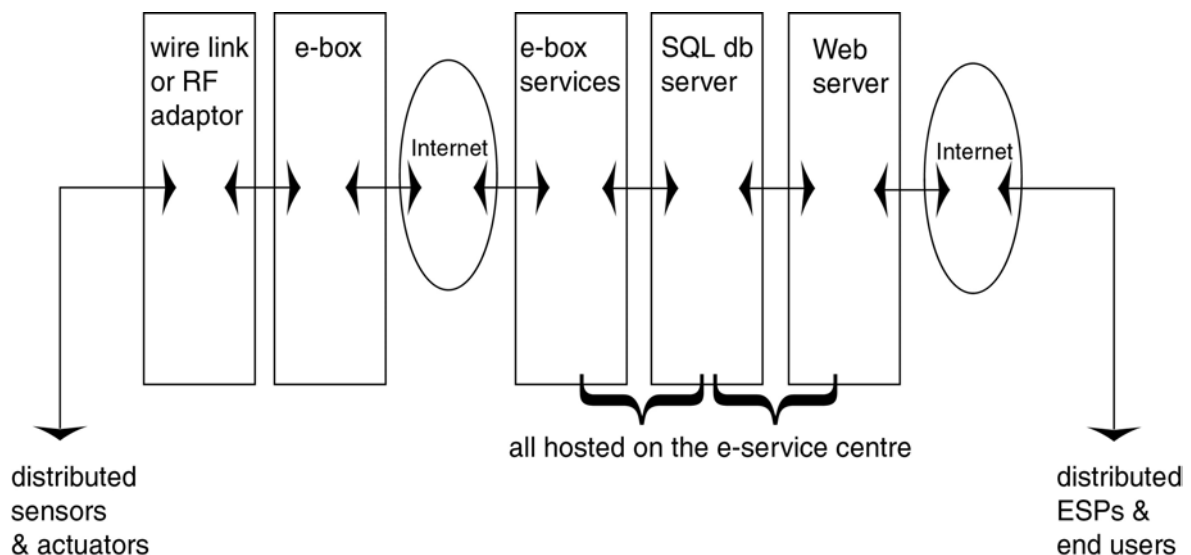
Figure 1 Components of the SmartHomes System
