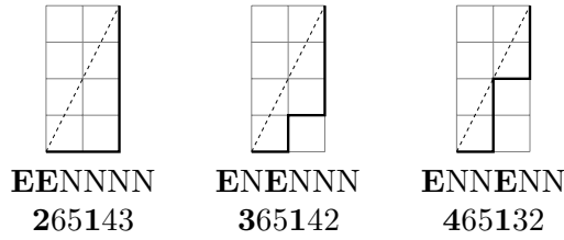
Fig. 4: \mathcal{S}_2^2(123) and corresponding lattice paths
