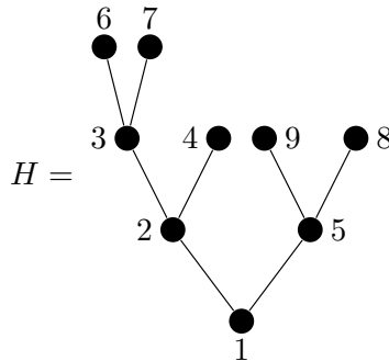
Fig. 1: A binary heap on 9 vertices
