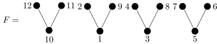
Fig. 3: A binary shrub forest with 12 vertices
