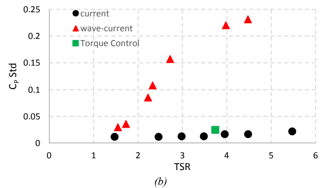
Fig. 6 Standard deviation of the power coefficient of the turbine working during extreme wave-current events (red and blue) and during current alone (black) at a) 0.5m/s and b) 1 m/s.
