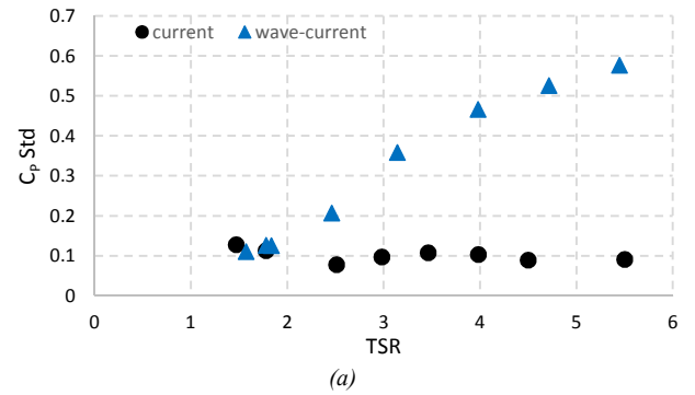
Fig. 5 Power coefficient of the turbine during extreme wave-current events (red and blue) and during current alone (black) at a) 0.5m/s and b) 1 m/s.
