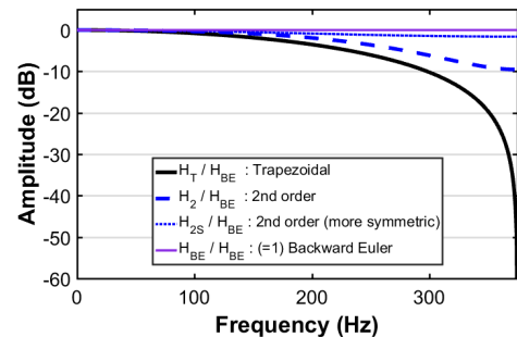
Fig. 7 Curve fitting expression H_{I_{vv}}/H_{I_{BE}} response, f_s=750 Hz.
