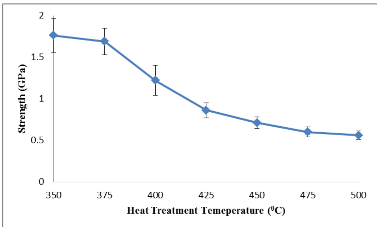
Figure 3 Heat Treated GF Strength
