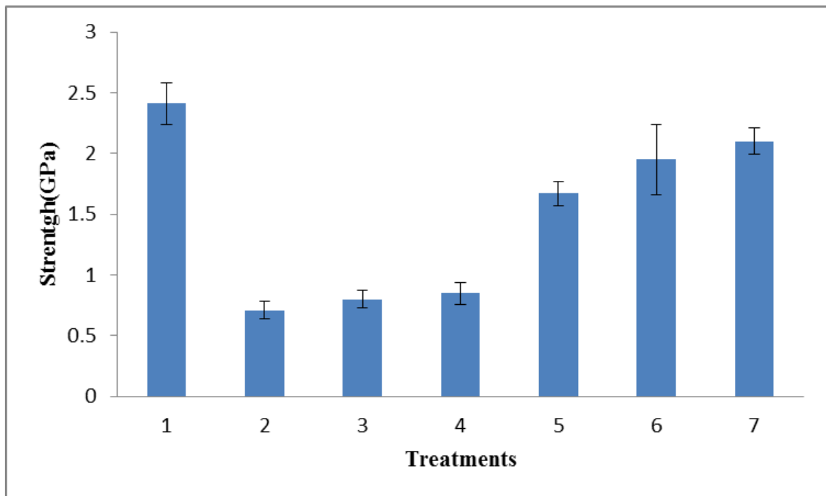
Figure 4 Average Fibre Strength
