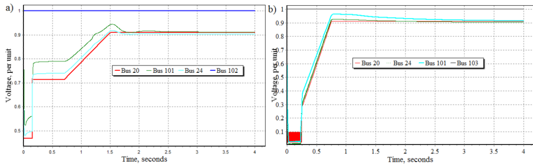
Fig. 7. voltage responses at several busses (a) E.ON voltage dip at Bus 20; (b) Nordic voltage dip at Bus 20
