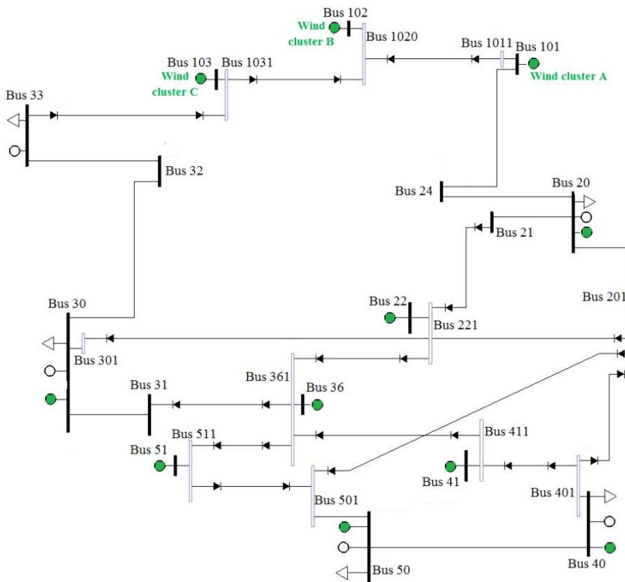
Fig. 3. Benchmark system single line diagram
