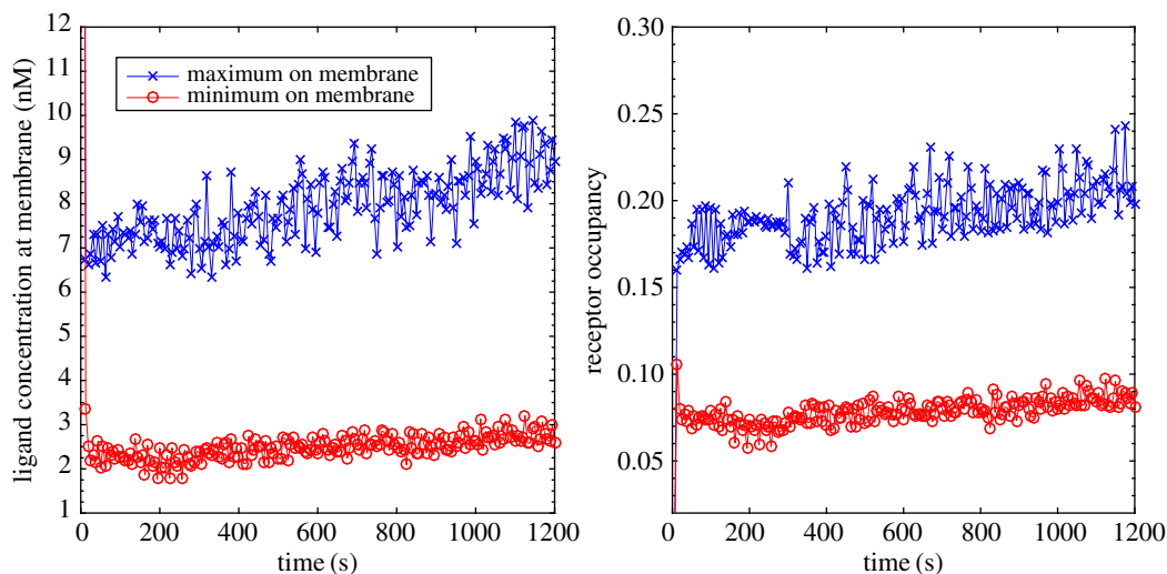
Figure 5. Computed ligand concentration and receptor occupancy on the membrane of an evolving cell in a shallow linear chemotactic field.
