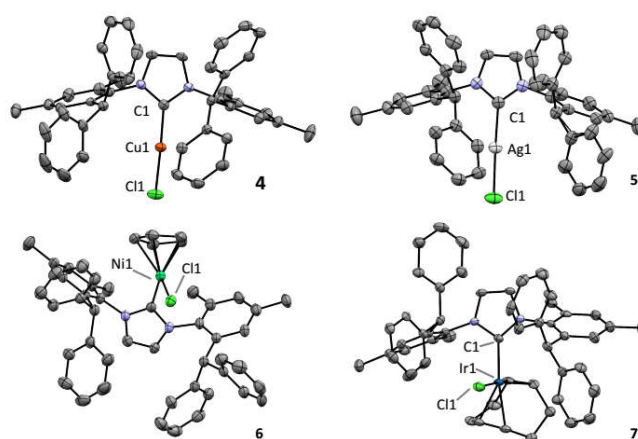
Figure 3. Molecular structures of complexes 4–7 as determined by X-ray diffraction. H atoms, minor disorder components, and solvent molecules are omitted for clarity.
