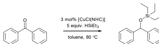
Scheme 4. The hydrosilylation test reaction.
