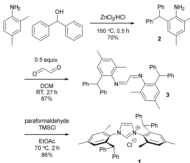
Scheme 1. Synthesis of the new NHC ligand.
