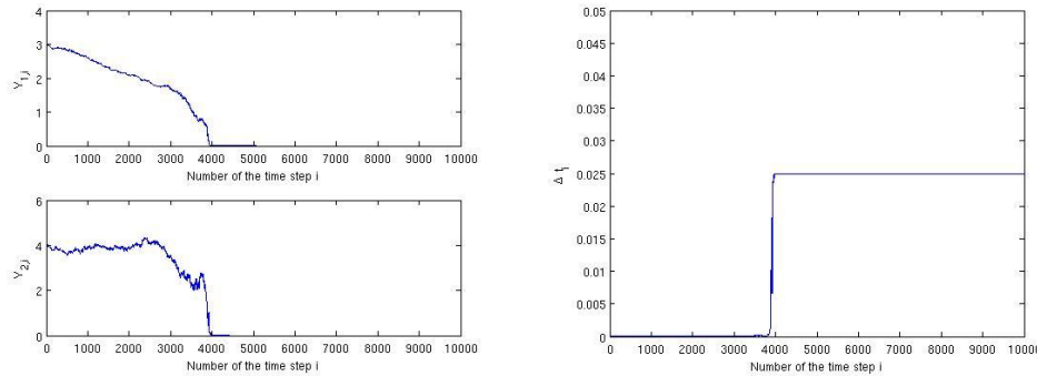
Figure 2: Left: One simulation path of Y_{1,\cdot} and Y_{2,\cdot} , Right: The stepsize of each time step.
