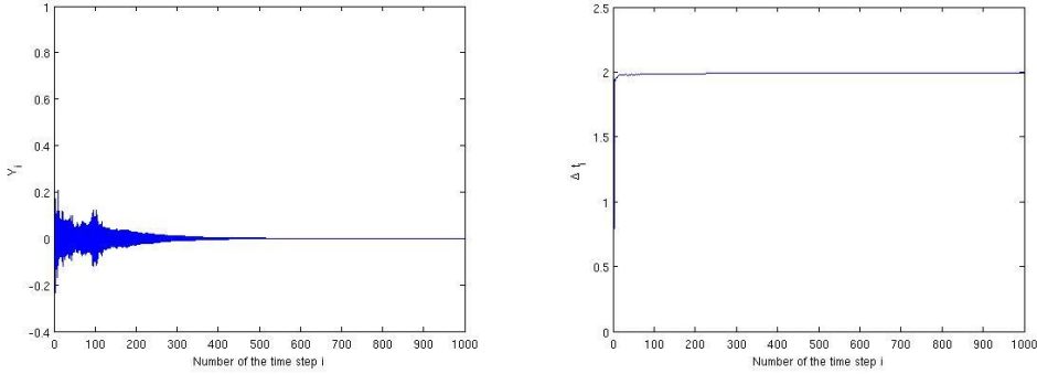
Figure 1: Left: One simulation path, Right: The stepsize of each time step
