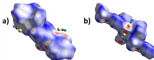
Figure 10. Hirshfeld surfaces mapped with d_{\text{norm}} for a) a molecule of 3 and b) an extended monomer of 6 showing the tetrel bonding between the Pb atoms (within the surface) and thiocyanate anions
