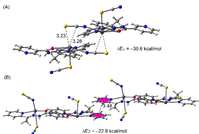
Figure 13. Theoretical models used to analyse the tetrel bonding interactions in compound 3 . Distances in Å.
