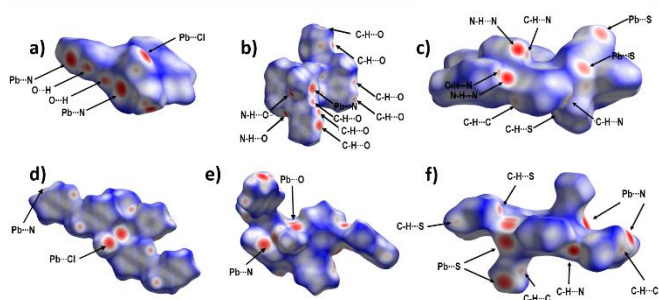
Figure 7. Hirshfeld surfaces mapped with d_{\text{norm}} for a) 1 , b) 2 , c) 3 , d) 4 , e) 5 and f) 6 .
