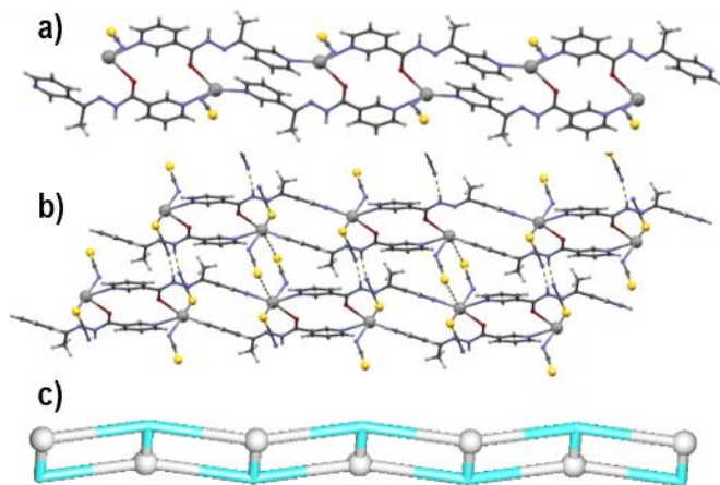
Figure 6. Structural fragments of 6 . (a) Cationic metal-organic [\text{PbL}_2(\text{SCN})]_n^{n+} chain with H-bonded \text{SCN}^- anions. (b) Binding of [\text{PbL}_2(\text{SCN})]_n^{n+} chains and \text{SCN}^- counter-ions into 2D sheets perpendicular to the [101] direction by supramolecular \text{Pb}\cdots\text{S} and \text{Pb}\cdots\text{C} interactions. (c) Topological representation of a simplified underlying 1D network showing a uninodal 3-connected metal-organic chain with the SP 1-periodic net (4,4)(0,2) topology; colour codes: 3-connected Pb1 nodes (grey balls), centroids of 3-connected \mu_3\text{-L2} nodes (cyan); rotated view along the a axis.
