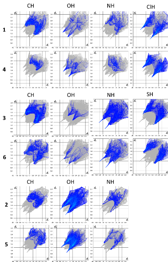
Figure 9. Decomposed fingerprint plots showing the main types of intermolecular contacts in structures of 1-6 .
