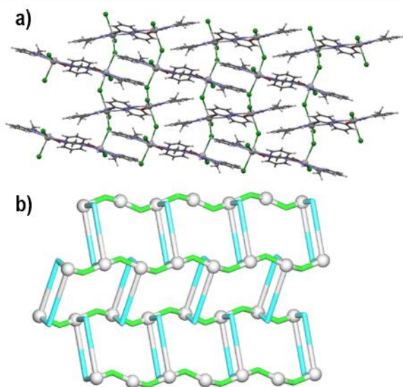
Figure 1. Structural fragments of 1 viewed along the a axis. (a) 2D metal-organic network. (b) Topological representation of a simplified underlying network showing a uninodal 4-connected metal-organic layer with the hcb [Shubnikov hexagonal plane net/(6,3)] topology; colour codes: 4-connected Pb1 nodes (grey balls), centroids of 2-connected \mu_2 -L1 (cyan) and \mu_2 -Cl (green) linkers.
