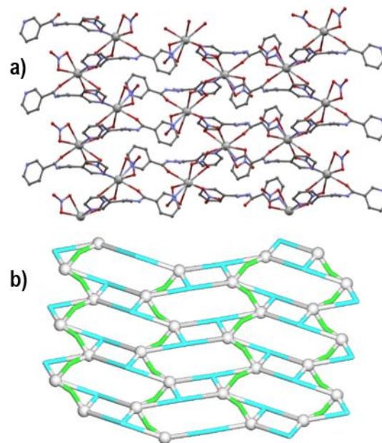
Figure 5. Structural fragments of 5 viewed along the a axis. (a) 2D metal-organic network (hydrogen atoms were omitted for clarity). (b) Topological representation of a simplified underlying 2D network showing a binodal 3,5-connected metal-organic layer with the gek1 topology; colour codes: 5-connected Pb1 nodes (grey balls), centroids of 3-connected \mu_3 -L2 nodes (cyan), and centroids of 2-connected \mu_2 -NO 3 linkers (green).
