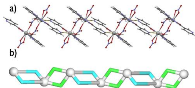
Figure 2. Structural fragments of 2 viewed along the c axis. (a) Binding of the [\text{PbL1}(\text{NO}_3)_2]_2 units into a zigzag 1D metal-organic chain (elongated Pb...N bonds are drawn as stippled lines). (b) Topological representation of a simplified underlying network showing a uninodal 2-connected chain with the 2C1 topology; colour codes: 2-connected Pb1 nodes (grey balls), centroids of 2-connected \mu_2 -L1 (cyan) and \mu_2 -Cl (green) linkers.
