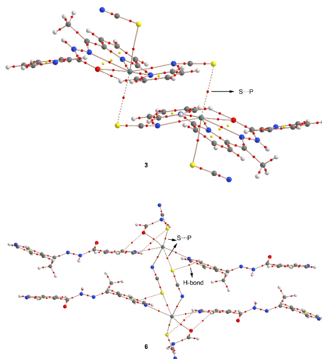
Figure 15. AIM distribution of bond and ring critical points (red and yellow spheres, respectively) in compounds 3 and 6 . The bond paths connecting bond critical points are also shown.
