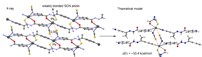
Figure 14. Left: Partial view of the X-ray structure of compound 6 . Right: Theoretical model used to analyse the tetrel bonding interactions in compound 6 . Distances in Å.
