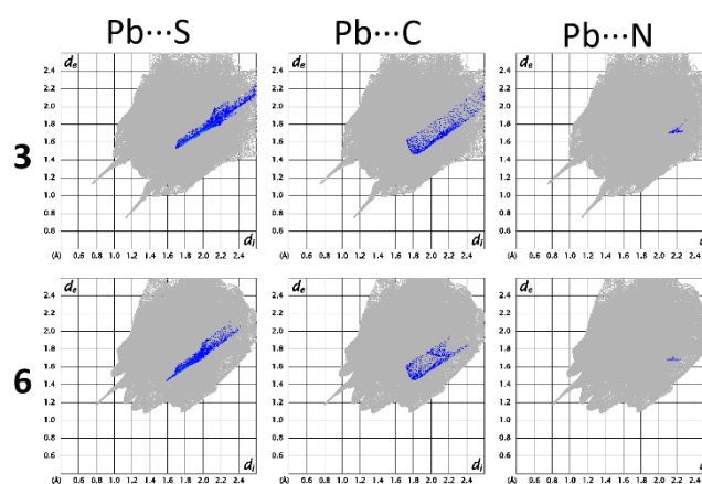
Figure 11 Decomposed fingerprint plots showing contacts including Pb in 3 and 6 .
