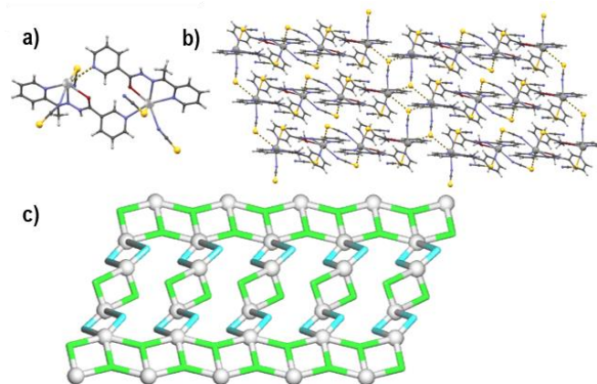
Figure 3. Structural fragments of 3 . (a) A non-centrosymmetric [\text{PbL1}(\text{SCN})_2]_2 dimeric unit (a) long intramolecular Pb...N contact is drawn as a stippled line. (b) Binding of [\text{PbL1}(\text{SCN})_2]_2 dimers into a supramolecular 2D sheet perpendicular to [101] direction (intermolecular Pb...S contacts are drawn as stippled lines). (c) Topological representation of a simplified underlying network showing a binodal 3,4-connected supramolecular layer with the 3,4L83 topology; colour codes: Pb1 nodes and Pb2 linkers (grey balls), centroids of L1 linkers (cyan), and centroids of SCN nodes and linkers (green); view along the c axis.
