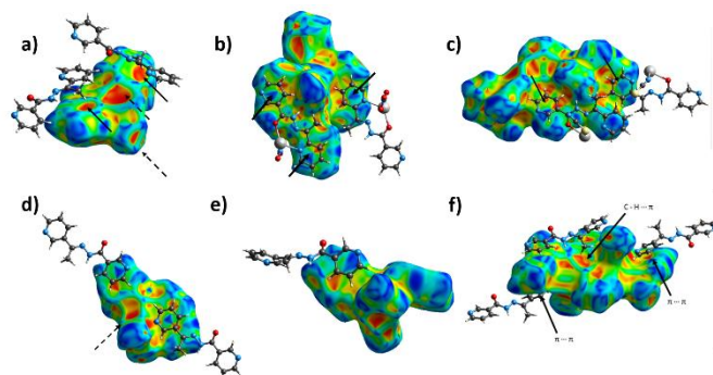
Figure 8. Hirshfeld surfaces mapped with shape index function for a) 1 , b) 2 , c) 3 , d) 4 , e) 5 and f) 6 . Dashed arrows denote parts of the surface corresponding to covalent bonds in polymeric compounds. Full arrows mark \pi stacking interactions, unless stated differently.
