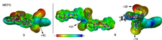
Figure 12. MEPS of compounds 3 and 6 at the B3LYP/6-31+G* level of theory.
