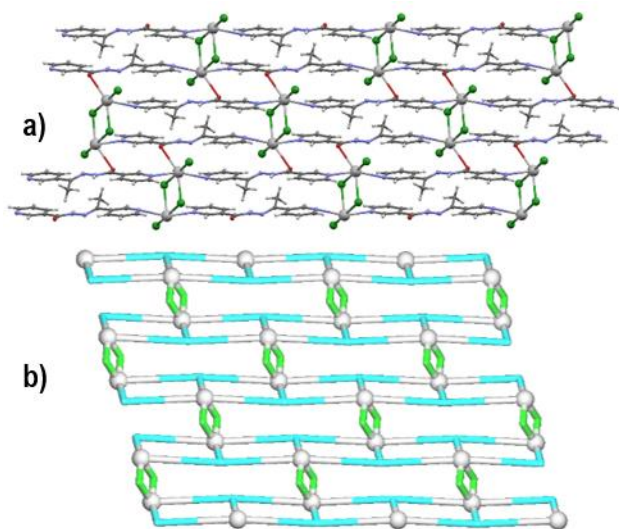
Figure 4. Structural fragments of 4 viewed along the a axis. (a) 2D metal-organic network. (b) Topological representation of a simplified underlying 2D network showing a binodal 3,4-connected metal-organic layer with the 3,4L83 topology; colour codes: 4-connected Pb1 nodes (grey balls), centroids of 3-connected \mu_3 -L2 nodes (cyan), and centroids of 2-connected \mu_2 -Cl linkers (green).
