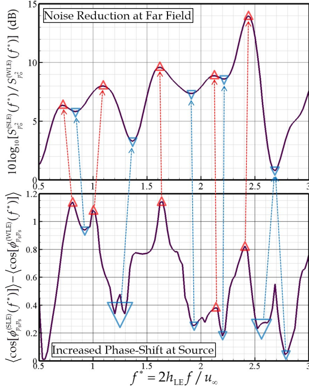
FIGURE 25. Relative difference in phase spectra between SLE and WLE cases compared with the radiated noise-reduction spectrum. Symbols denote the local maxima ( \triangle ) and minima ( \nabla ) of each spectra profile.
