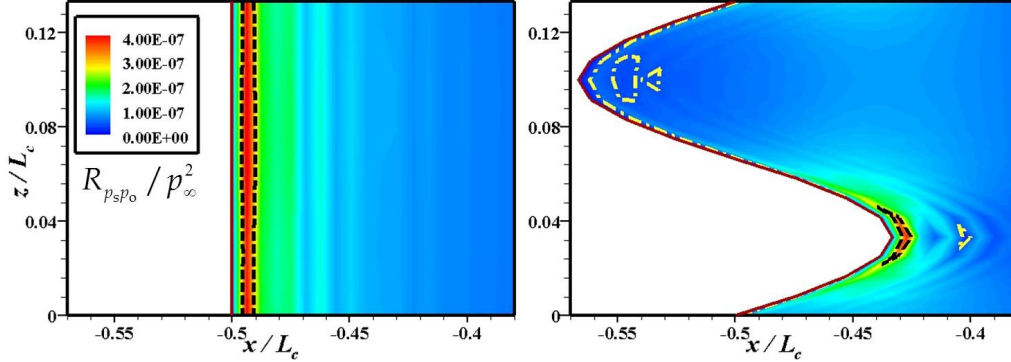
FIGURE 14. Contour plots of two-point correlation R_{p_s p_o}(\mathbf{x}_s; \mathbf{x}_o) between the surface pressure fluctuations and the radiated far-field sound at an observer point \mathbf{x}_o = (0, 5L_c, 0) , for the SLE (left) and the WLE (right) cases. The two-point correlation is based on (2.13). The dashed and the dash-dotted lines represent contour lines that enclose the region of R_{p_s p_o} / p_\infty^2 \geq 3 \times 10^{-7} and R_{p_s p_o} / p_\infty^2 \leq 4 \times 10^{-8} , respectively.
