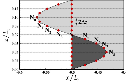
FIGURE 15. Illustration of the current probe points along the LE to obtain time signals of \Delta p_s^i and calculate the auto- and cross-spectra from the Peak ( N_0 ) to the Root ( N_8 ). The actual probe points are located on the second grid line from the LE where the source strength is maximum.
