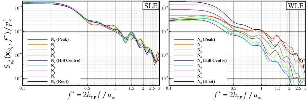
FIGURE 16. Auto-spectra of surface pressure fluctuations along the LE; S_{p_s^2}(\mathbf{x}_{N_i}, f) for i = 0, \dots, 8 ; obtained at the probe points denoted in figure 15, for the SLE (left) and WLE (right) cases. The WLE case is for h_{LE}/L_c = 1/15 and \lambda_{LE}/L_c = 2/15 .
