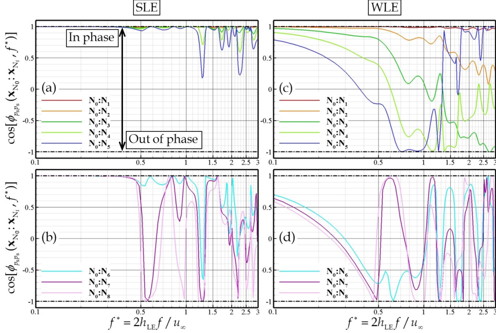
FIGURE 22. The profiles of \cos[\phi_{psps}(\mathbf{x}_{N_0}:\mathbf{x}_{N_i}, f^*)] where \phi_{psps}(\mathbf{x}_{N_0}:\mathbf{x}_{N_i}, f) is the two-point phase spectrum of surface pressure fluctuations between the Peak ( N_0 ) and one of the remaining probe points ( N_1, \dots, N_8 ) denoted in figure 15, for the SLE (left) and WLE (right) cases. The WLE case is for h_{LE}/L_c = 1/15 and \lambda_{LE}/L_c = 2/15 .
