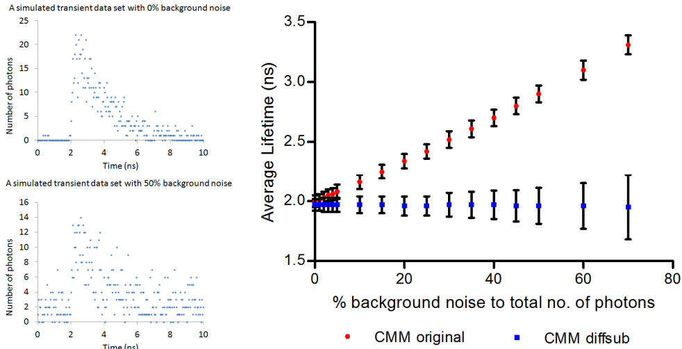
Fig.7 Analysis of simulated transient datasets showing how increasing the percentage contribution background noise to total number of photons affected the average lifetime value of 4096 transients determined using CMM original and CMM diffsub . For each individual transient, the total number of photons remains constant at 1000 counts.
