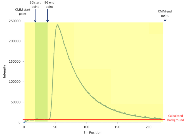
Fig. 6. A typical graph of a measured fluorescence histogram indicating the typical positions of the timing windows for measurement (yellow) and background (green) when set up to acquire data for CMM_{diffsub} .
