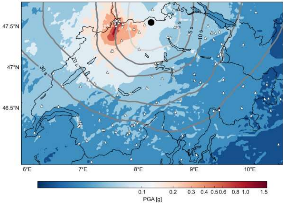
Figure 3 - PGA shaking scenario for the Basel 1356 M_w 6.6. event, computed as described in the text. The grey curves are contour lines of expected lead-times at the NPP of Beznau (the black circle) based on the geometry of the Swiss national seismic network and a minimum number of 6 station triggers to declare the onset of the seismic event.
