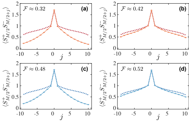
FIG. 4: Comparison of correlations and state fidelity in the presence of spontaneous emission— \langle S_i^+ S_{i+j}^- \rangle correlations for the adiabatically prepared state with U_{AB}/U = 0.97 in a system with 40 particles on 20 sites, compared to the ground-state correlation (dashed lines). The parameter values here are indicated as circles in Fig. 3d. (a/b): High spontaneous emission rate, \gamma = 10^{-3}J , (c/d) low spontaneous emission rate \gamma = 10^{-4}J . Panels (a) and (c) are for a faster ramp with t_a J = 38.9 , (b) and (d) for the slower ramp with t_a J = 117.5 . The state-fidelities are given in the plots.
