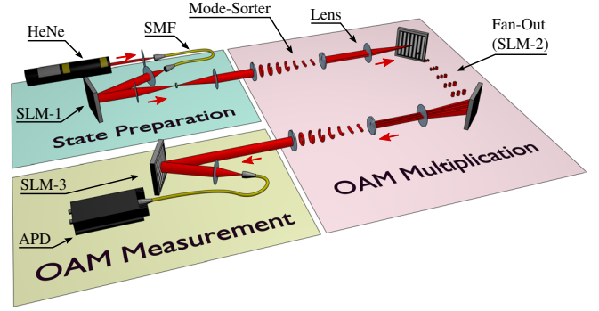
FIG. 2 (color online). Experimental schematic. —A HeNe laser beam, spatially filtered with a single mode fiber (SMF) and collimated, is directed onto a phase-only spatial light modulator (SLM-1) to generate the desired combination of input OAM eigenmodes. The beam is then sent through a pair of machined polymer refractive elements that comprise the first OAM sorter. The optical field at the output plane of this sorter is imaged onto the top half of a second SLM implementing a fan-out grating. The fan-out was set to produce three copies of the beam, resulting in a \times 3 multiplication of the OAM quantum number of each mode. The Fourier plane of this grating is imaged onto the bottom half of the same SLM displaying the appropriate hologram to correct for the relative phase between the three copies. The three copies are then demagnified by a cylindrical lens and injected through a second OAM sorter operated in reverse. We measured the OAM spectrum of light at the output of the multiplier using a series of projective measurements for various values of \ell , which were implemented using a third SLM and a single-mode-fiber-coupled avalanche photodiode (APD).
