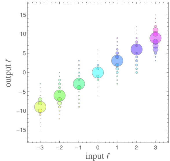
FIG. 4 (color online). OAM multiplication performance. —For each input eigenmode we measure the composition of the multiplied output. Circle size is linearly proportional to the overlap with the output modes. As can be seen, the small leakage onto the neighboring output modes is contained within a few adjacent modes. A sufficiently distant input superposition such as |3\rangle + |-3\rangle would maintain an effective orthogonality.
