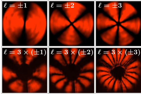
FIG. 3 (color online). Coherent OAM multiplication. —Top row: Near field of input coherent superpositions. Bottom row: Tripled output states. The number of petals is 6|\ell| , as expected from a coherent operation.
