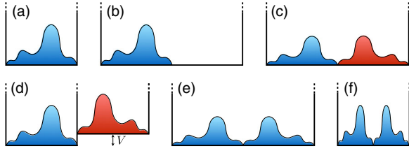
FIG. 1 (color online). Hilbert hotel protocol .—(a) The initial state is a single particle wave function \psi(x) within an infinite square potential well. (b) We instantaneously expand the well to twice its original width. The original wave function is not immediately changed but the eigenbasis is different. (c) We allow free evolution for a period corresponding to the original fundamental period. The wave function is reflected around the center of the expanded well, with an undesired phase shift. (d) We insert an infinite barrier in the center (where the wave function is zero) to split it into two independent wells that evolve separately, an energy shift on one well corrects the relative phase. (e) After the phase correction we align the potentials and merge the two halves back together. (f) An adiabatic compression of the well maps the eigenstates of the expanded well to those of the original well. The original wave function has now been halved and reflected, corresponding to the Hilbert hotel operation \hat{\mathbb{H}}_2 being applied to the eigenstates \psi(x) .
