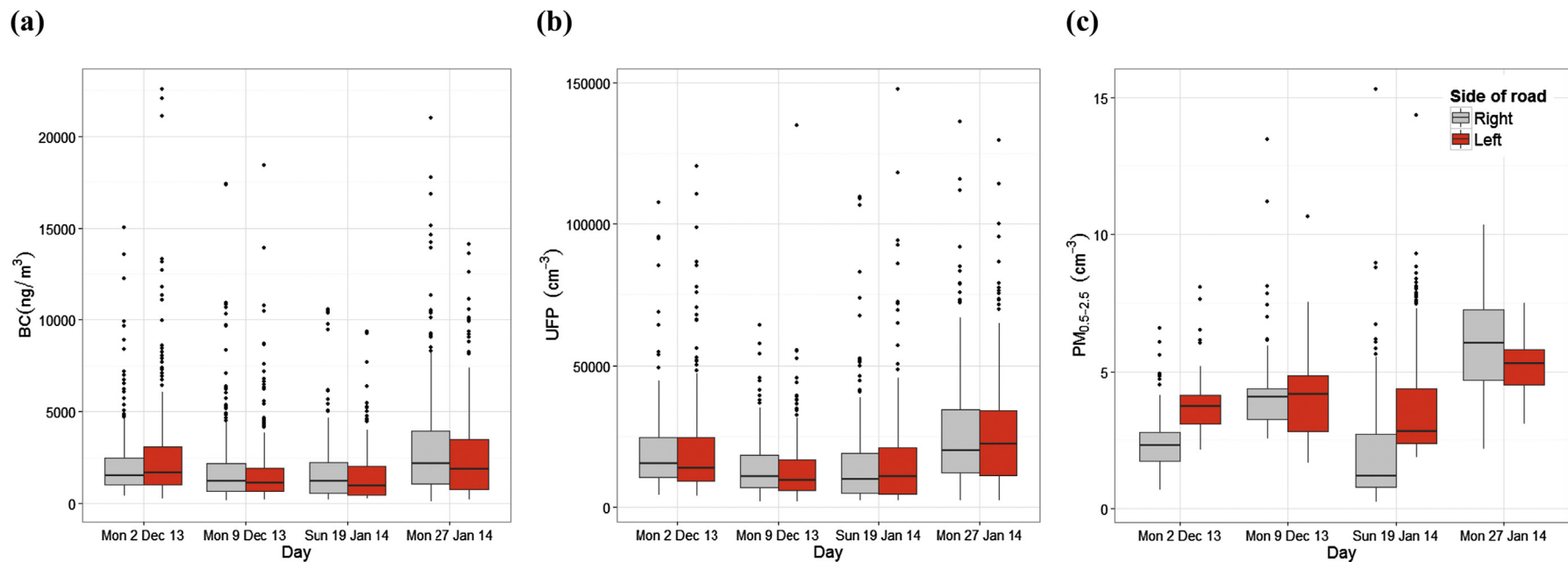
Fig. 2. Distributions of (a) BC, (b) UFP and (c) PM_{0.5-2.5} concentrations measured on both sides of the road during each week in the winter campaign. The bold horizontal line denotes the median, and the box demarcates the interquartile range. The whiskers extend to the values 1.5 times the IQR on each side of the median. The PM_{0.5-2.5} concentration measured by one of the DylOs instruments was corrected based on the statistics from MA regression analysis of instrument co-deployment during the winter campaign (Table S2). Side of road is defined with respect to the walking direction in the mobile measurements. The UFP concentrations in (b) are 1 min averages of the raw 1 s data.
