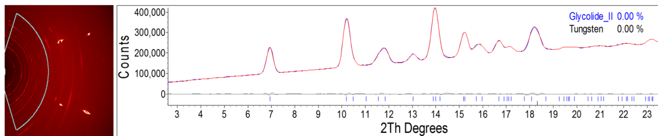
Fig 4 – Diffraction image (left) and powder diffraction pattern (right) of glycolide Form 2. The bright spots in the diffraction image are caused by the diamonds of the DAC. The diffraction rings at high 2-theta angle are caused by the tungsten gasket. The Pawley fit of the data fits very well with the calculated pattern from the single crystal data ( R_{wp} = 0.79\% ).
