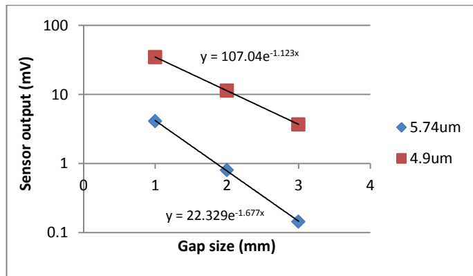
Figure 8 Sensor output vs. gap size, old oil
