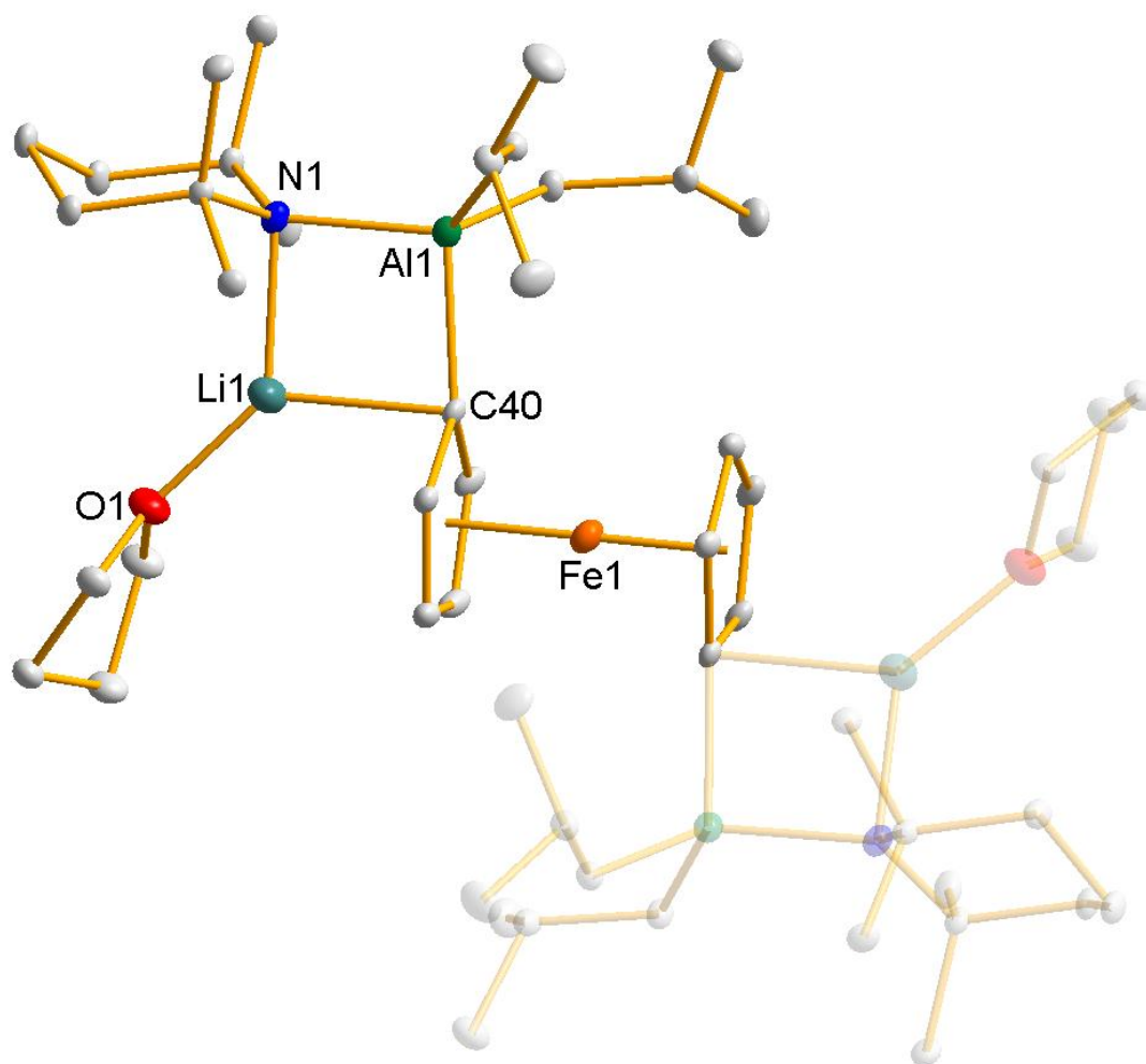
Figure 8 Molecular structure of the dialuminated ferrocene [THF·Li(μ-TMP)Al( i Bu) 2 ] 2 (C 5 H 4 ) 2 Fe ( 5 ). Ellipsoids are shown at 50% probability level and all hydrogen atoms have been removed for clarity. Symmetry operation to generate second half of structure: 2.5-x, y, 2-z. Selected bond lengths (Å) and angles (°): Al1-
