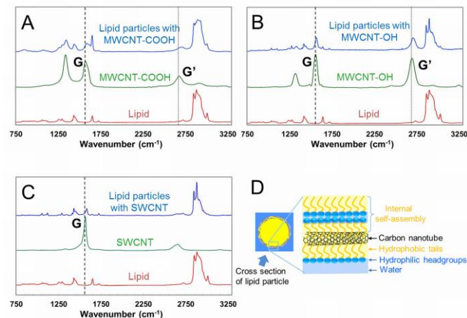
Fig 3 Raman spectra elucidating lipid decoration on CNTs Raman spectra of (A) pure lipid, MWCNT-COOH and CNT stabilized lipid nanoparticles containing 5.0 \mu\text{g}/\text{ml} MWCNT-COOH, (B) pure lipid, -OH functionalized multi-walled carbon nanotubes (MWCNT-OH) and lipid nanoparticles containing 5.0 \mu\text{g}/\text{ml} MWCNT-OH, and (C) pure lipid, single-walled carbon nanotubes (SWCNT) and lipid nanoparticles containing 0.3125 \mu\text{g}/\text{ml} SWCNT (Other concentrations’ Raman spectra are shown in ESI Fig. S1). All curves represent an average of ten spectra where intensities, in arbitrary units (labels not shown) are plotted along y-axis. Blue shift in typical G and G’ bands of CNTs represent the interaction between CNT surface and lipid molecules. Lipid decoration over CNTs was also depicted by decrease in relative intensities of CNT peaks and appearance of lipid signals which are visible from blue curves. Dashed (G band) and dotted (G’ band) lines are used to guide the eyes. (D) Schematic diagram of lipid self-assembling on CNT surface. Alkyl chains of lipid molecules interact with hydrophobic CNT surface whereas the hydrophilic lipid headgroups face aqueous region. Interior of particles is filled with self-assembled lipid nanostructure as indicated by the cross section of lipid particle (yellow).
