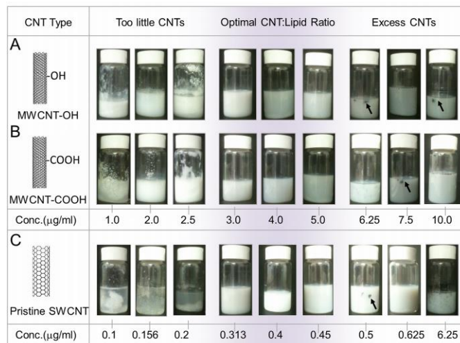
Fig. 4 Optimum CNT concentrations for stable emulsions Stable emulsions (shown by purple shade) were obtained in the region of 3.0-5.0 \mu\text{g}/\text{ml} for MWCNT-OH as in (A) and MWCNT-COOH as in (B). The concentration of SWCNTs for stable emulsions as in (C) was about an order of magnitude less than above numbers. It was also possible to get stable emulsions at concentrations very near to these ranges (as indicated by color gradient). For lower concentrations of CNTs, large domains of lipid were seen as there were too little CNTs per lipid whereas for higher concentrations there were too many CNTs which tend to aggregate; some of these are indicated by black arrows.
