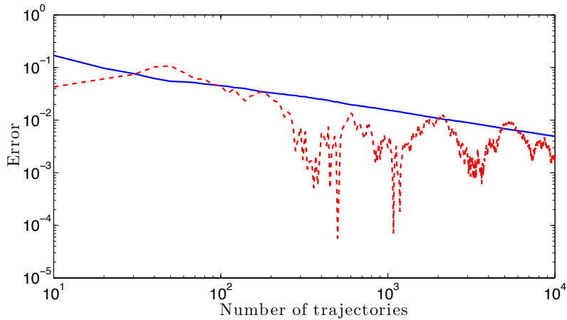
FIG. 4: Statistical errors in the quantum trajectories computation for a two-level system. Here we compare the statistical error estimate (blue solid line) to the absolute error in the averaged value of P_e when compared with the exactly computed value (red dashed line) at a time t\Omega = 40 . We show these values as a function of the number of trajectories over which we average, with all quantities plotted on a logarithmic scale. As expected, the behaviour of both the statistical error and the discrepancy is somewhat erratic for small numbers of trajectories, but decrease steadily \propto 1/\sqrt{N} for larger numbers. The absolute error is mostly below the statistical error estimate, consistent with a gaussian distribution of possible errors with a standard deviation equal to our statistical error estimate. Note that these values depend on the particular random sample of trajectories obtained in the calculation. From the central limit theorem and the properties of Gaussian distributions that for any given computed values, we expect the absolute error to be smaller than the statistical error as it is quoted here for 68.2% of all possible samples.
