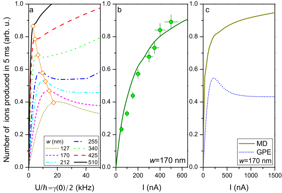
FIG. 27: a) Theoretical curves of the number of ions produced in 5 ms as a function of U/\hbar = \gamma_1(0) solving equation (84) for different values of the beam width w [122]. The values of U_M obtained using the approximate expression given in the text are shown as open diamonds over the corresponding curves. b) Number of ions measured after 5 ms of dissipation for a thermal cloud as a function of the EB current, with beam width w = 170(7) nm. The solid line is the result of the corresponding numerical simulation using the molecular dynamics method. c) Comparison between the theoretical curves of the number of produced ions as a function of I for the BEC and the corresponding classical analogue (beam width w = 170(7) nm) [122]. Reprinted figure with permission from G. Barontini, R. Labouvie, F. Stubenrauch, A. Vogler, V. Guarrera, and H. Ott, Phys. Rev. Lett. 110 , 035302 (2013). Copyright 2013 by the American Physical Society.
