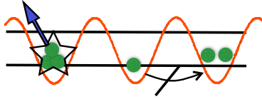
FIG. 23: Schematic showing the continuous quantum Zeno effect in the case of three-body loss in an optical lattice. If we have a large on-site rate of loss \gamma_3 , such that the tunnelling in the lowest Bloch band J \ll \gamma_3 , then tunnelling processes that populate a single site with three particles (i.e., where a particle on one site tunnels onto an already doubly-occupied site) will be suppressed. In this form, large on-site loss rates can counterintuitively lead to a reduction in the overall rate of loss, and can act as an effective dynamical interaction, which suppresses triple occupation.
