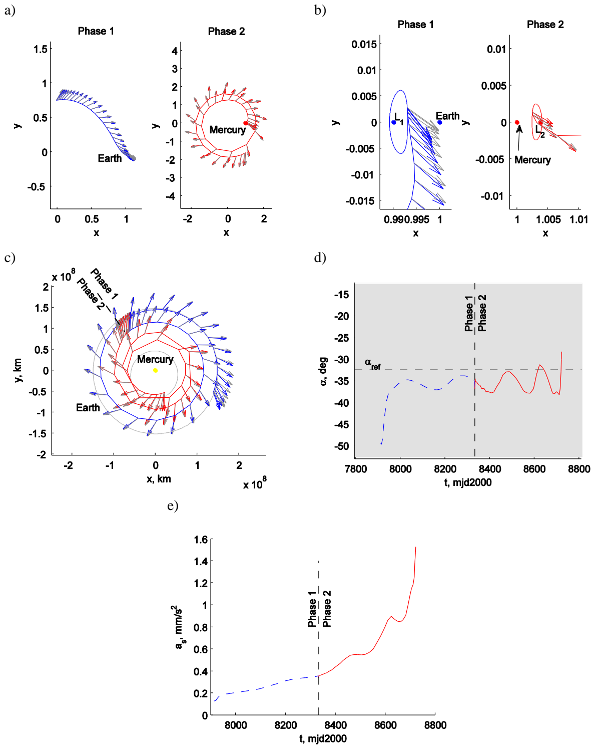
Figure 13 Earth- L_1 to Mercury- L_2 optimal solar sail transfer: details for \Delta\alpha = 20 deg. a) Transfer phases with sail acceleration direction (color) and optimal \hat{n}_{ref} -direction (grey). b) Detail of plot a). c) Transfer in heliocentric inertial reference frame. d) Cone angle. e) Solar sail acceleration magnitude.
