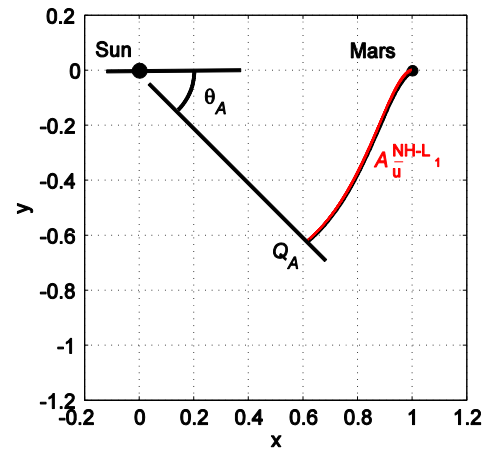
Figure 7 Earth- L_2 to Mars- L_1 first guess transfer. a, b) Departure conditions and design variables. c, d) Arrival conditions and design variables.
