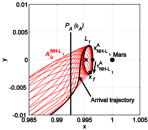
Figure 7 Earth- L_2 to Mars- L_1 first guess transfer. a, b) Departure conditions and design variables. c, d) Arrival conditions and design variables.
