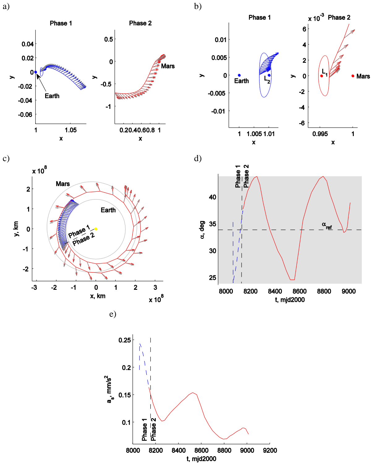
Figure 11 Earth-L 2 to Mars-L 1 solar sail transfer: details for \Delta\alpha = 10 deg. a) Transfer phases with sail acceleration direction (color) and optimal \hat{n}_{ref} -direction (grey). b) Detail of plot a). c) Transfer in heliocentric inertial reference frame. d) Cone angle. e) Solar sail acceleration magnitude.
