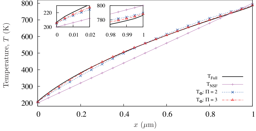
Figure 12: Final hybrid temperature solutions T_\Phi , along with the initial NSF temperature solution T_{NSF} , and the full DSMC temperature solution T_{Full} . Insets show results close to each wall.
