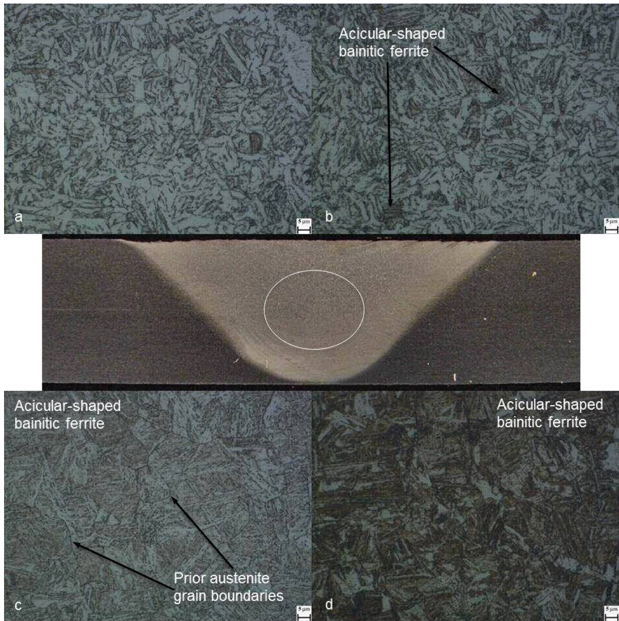
Fig. 3. Microstructure of mid-TMAZ [x1000, Etched] (a) 100 mm/min; (b) 120 mm/min; (c) 350 mm/min; (d) 375 mm/min.
