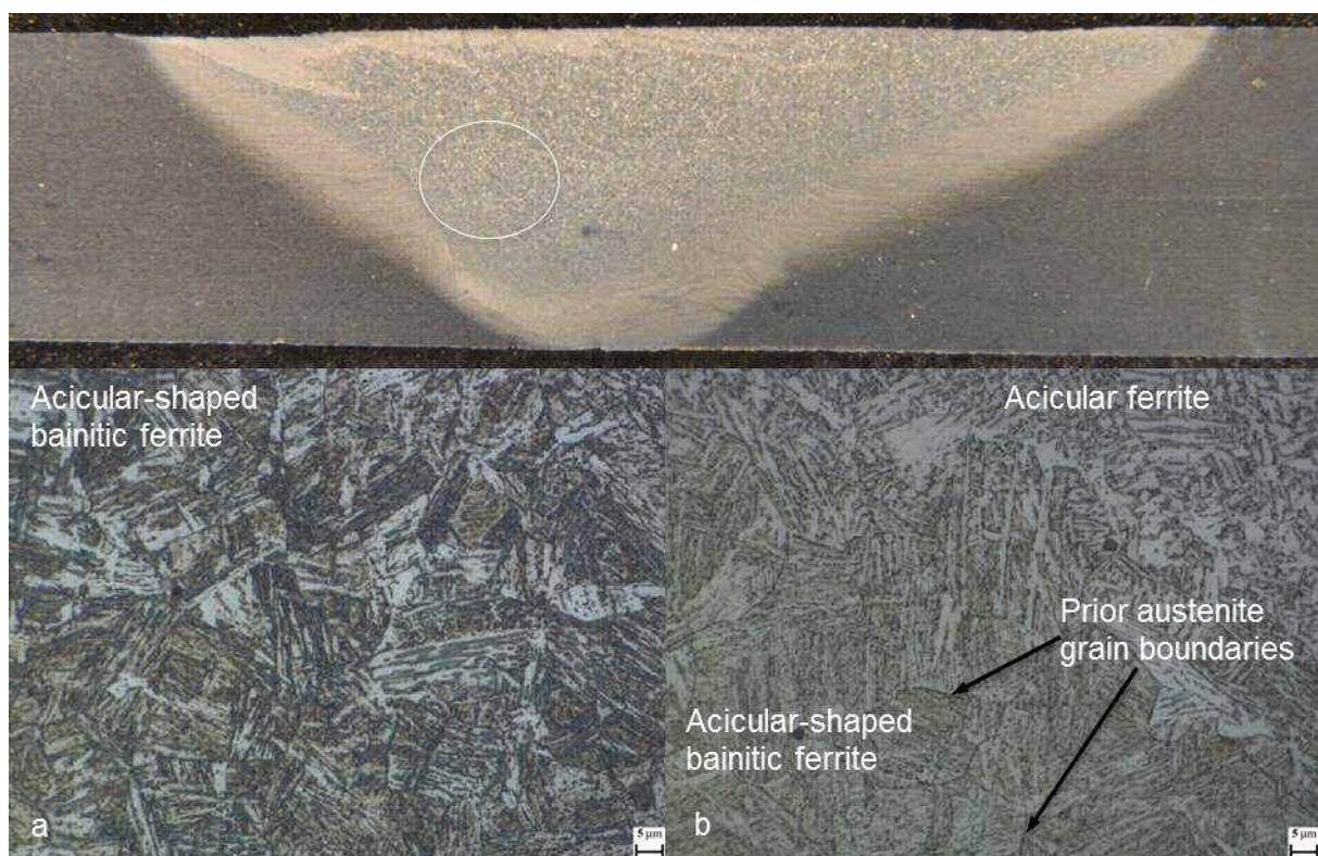
Fig. 4. Microstructure of mid-TMAZ AD side at 500 mm/min [x1000, Etched] (a) 675 rpm; (b) 700 rpm.
