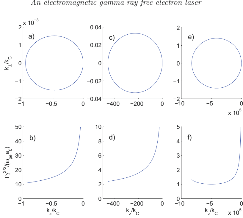
FIGURE 1. The resonant radiation wave vectors (top row) and the corresponding growth rates (bottom row) for a laser wiggler with 1\mu\text{m} wavelength ( k_0 = 6.28 \times 10^6\text{ m}^{-1} ) and amplitude a_0 = 1 , and for different gamma factors of the electron beam: \gamma_0 = 320 (left column), \gamma_0 = 0.71 \times 10^4 (middle column) and \gamma_0 = 0.71 \times 10^6 (right column).
